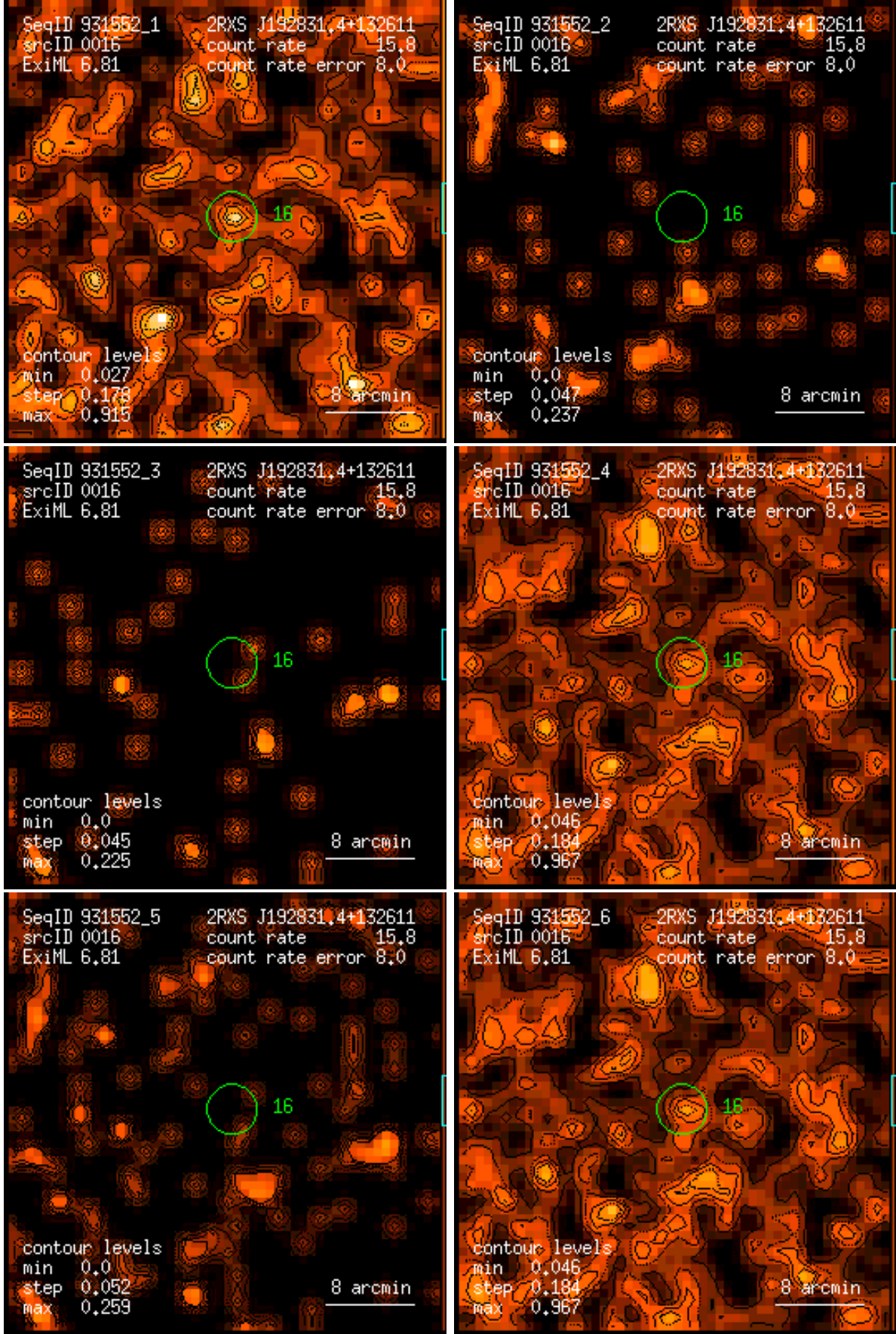
Figure 16: RASS 931552: detection 0016: band rate images, Gaussian filter: (1) PSPC channels 11 – 41, (2) 52 – 90, (3) 91 – 201, (4) 11 – 235, (5) 52 – 201, (6) 11 – 201. Broad band rates in counts/ks. Band rate contour levels in counts/ks/arcmin 2 .
