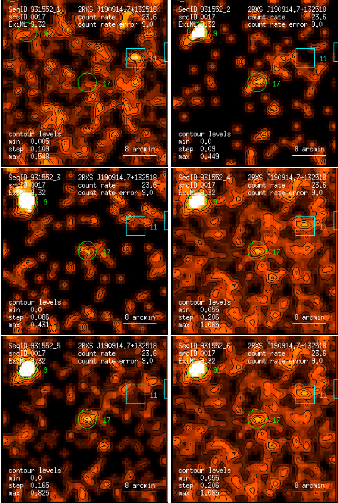
Figure 17: RASS 931552: detection 0017: band rate images, Gaussian filter: (1) PSPC channels 11 – 41, (2) 52 – 90, (3) 91 – 201, (4) 11 – 235, (5) 52 – 201, (6) 11 – 201. Broad band rates in counts/ks. Band rate contour levels in counts/ks/arcmin 2 .
