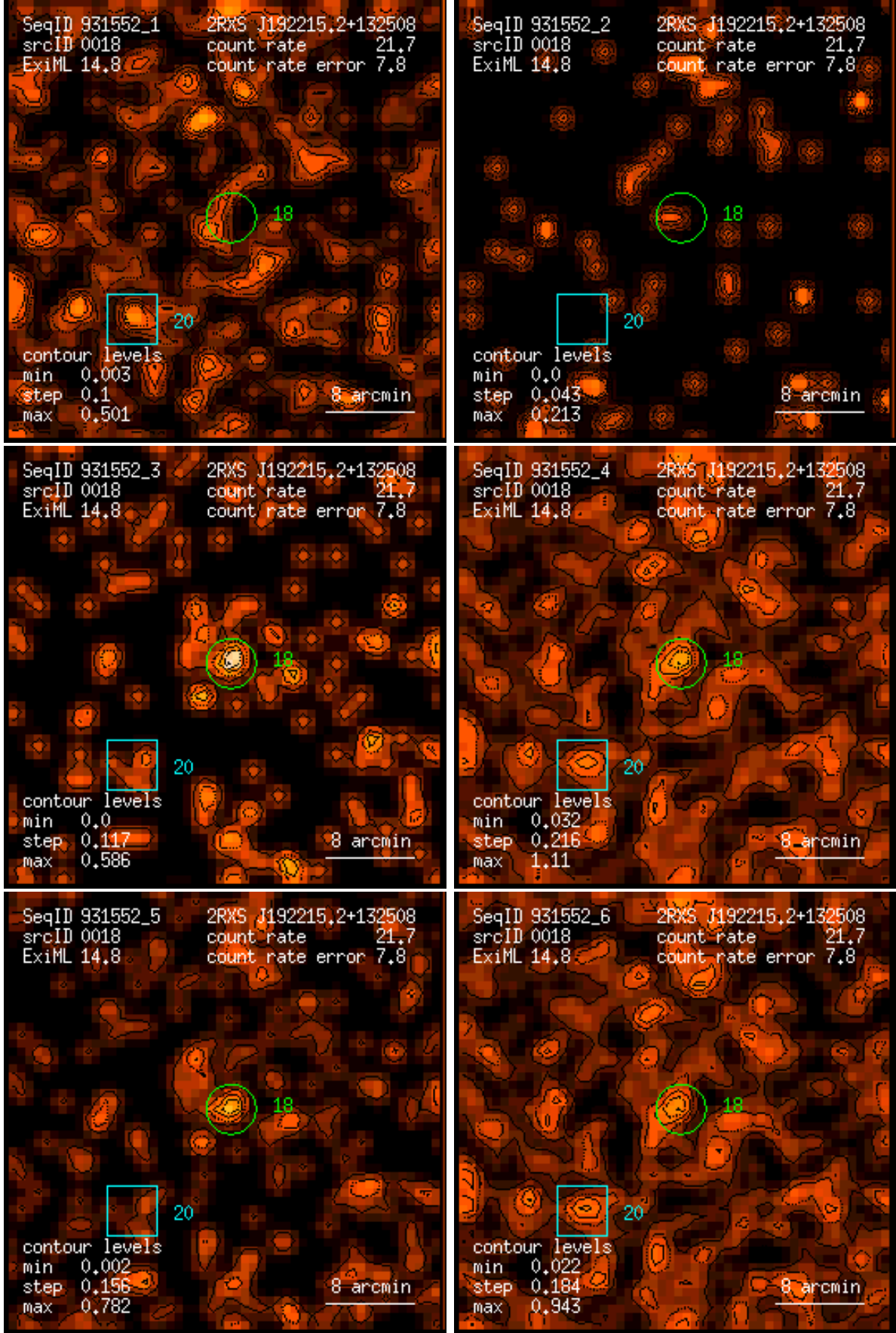
Figure 18: RASS 931552: detection 0018: band rate images, Gaussian filter: (1) PSPC channels 11 – 41, (2) 52 – 90, (3) 91 – 201, (4) 11 – 235, (5) 52 – 201, (6) 11 – 201. Broad band rates in counts/ks. Band rate contour levels in counts/ks/arcmin 2 .
