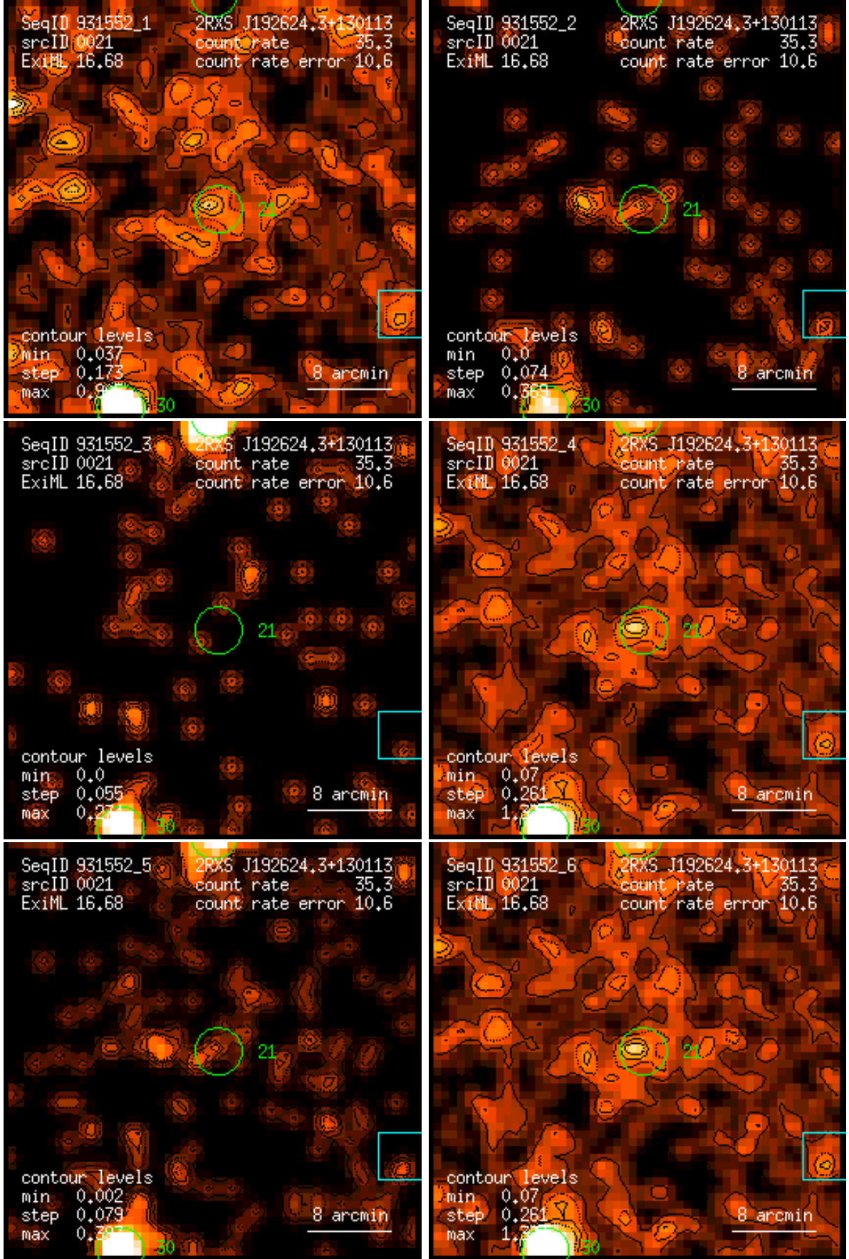
Figure 21: RASS 931552: detection 0021: band rate images, Gaussian filter: (1) PSPC channels 11 – 41, (2) 52 – 90, (3) 91 – 201, (4) 11 – 235, (5) 52 – 201, (6) 11 – 201. Broad band rates in counts/ks. Band rate contour levels in counts/ks/arcmin 2 .
