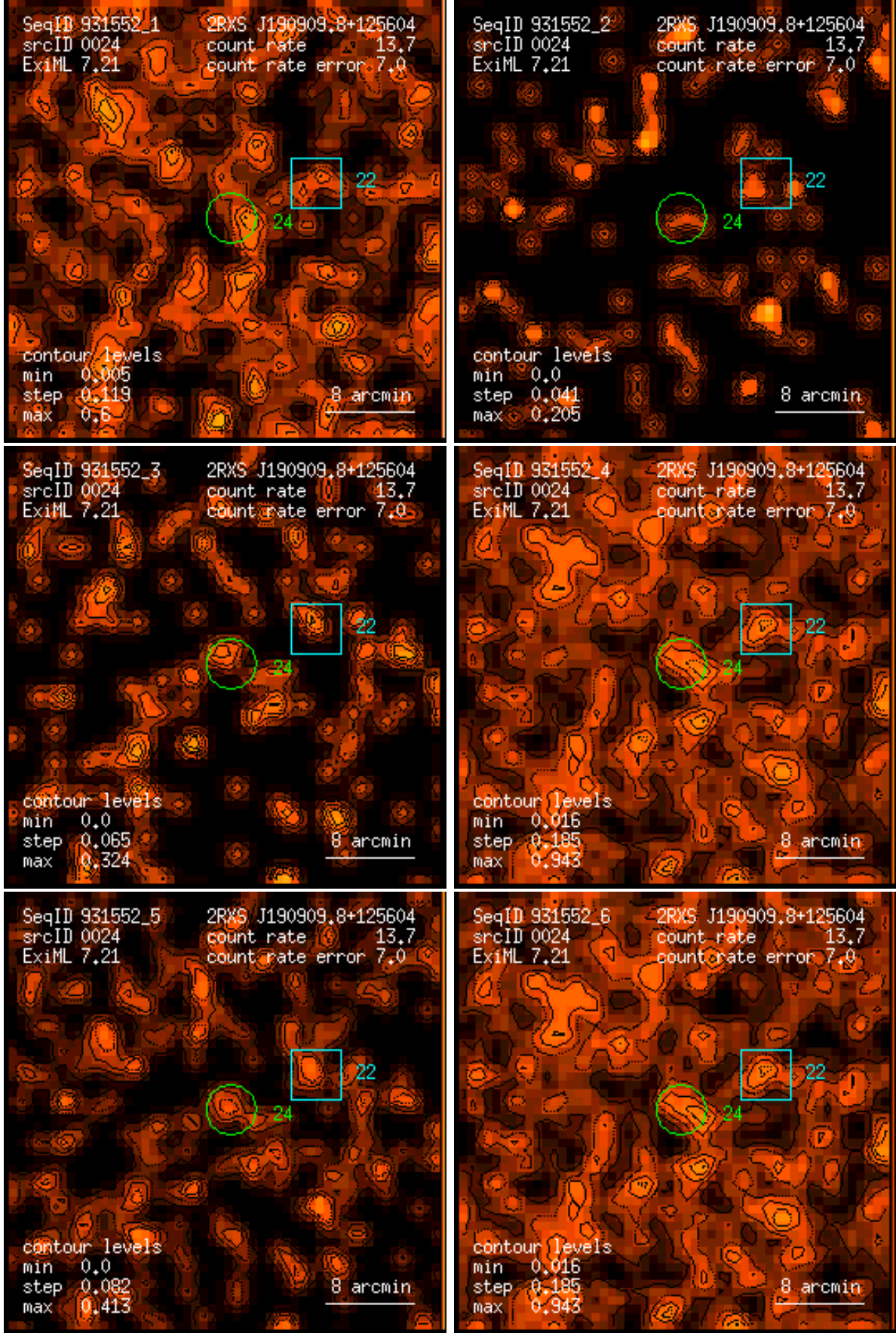
Figure 24: RASS 931552: detection 0024: band rate images, Gaussian filter: (1) PSPC channels 11 – 41, (2) 52 – 90, (3) 91 – 201, (4) 11 – 235, (5) 52 – 201, (6) 11 – 201. Broad band rates in counts/ks. Band rate contour levels in counts/ks/arcmin 2 .
