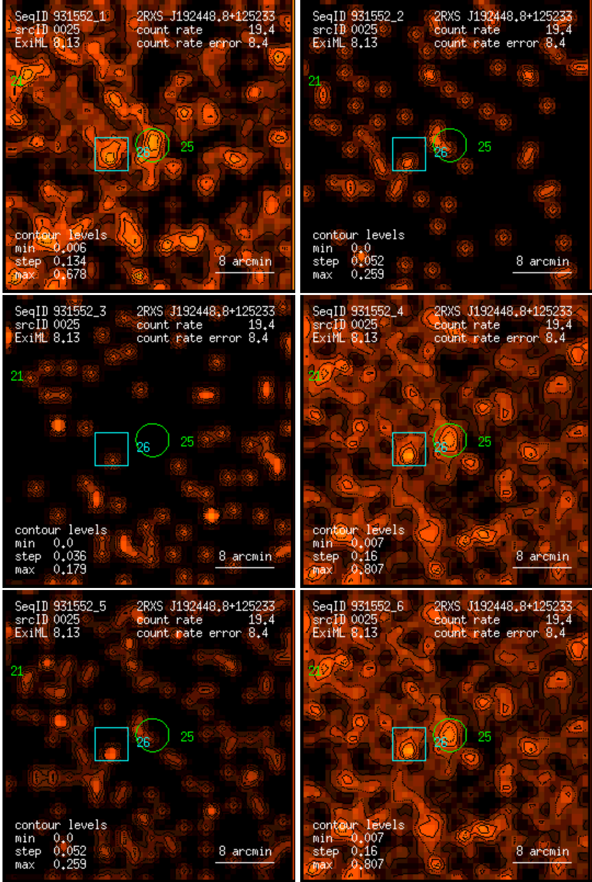
Figure 25: RASS 931552: detection 0025: band rate images, Gaussian filter: (1) PSPC channels 11 – 41, (2) 52 – 90, (3) 91 – 201, (4) 11 – 235, (5) 52 – 201, (6) 11 – 201. Broad band rates in counts/ks. Band rate contour levels in counts/ks/arcmin 2 .
