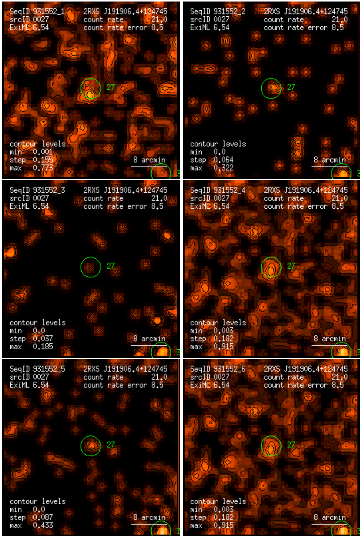
Figure 27: RASS 931552: detection 0027: band rate images, Gaussian filter: (1) PSPC channels 11 – 41, (2) 52 – 90, (3) 91 – 201, (4) 11 – 235, (5) 52 – 201, (6) 11 – 201. Broad band rates in counts/ks. Band rate contour levels in counts/ks/arcmin 2 .
