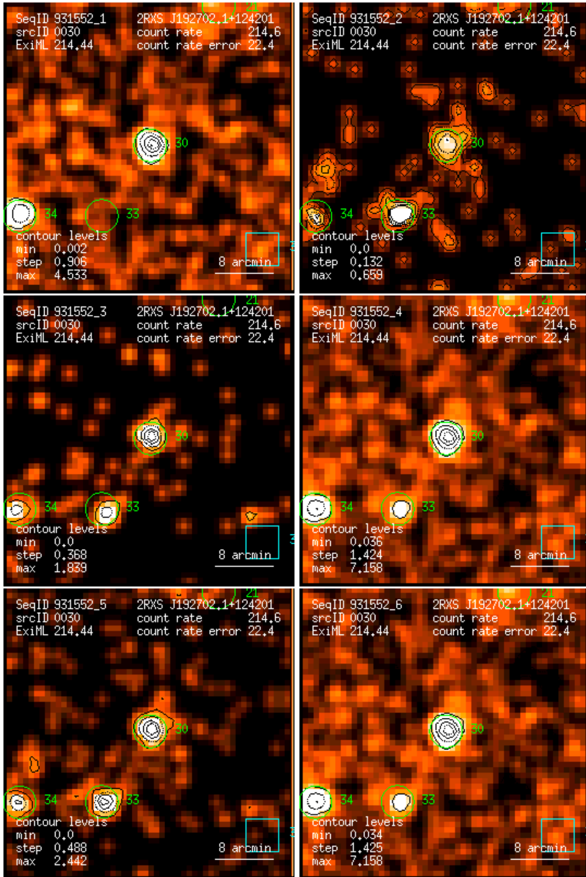
Figure 30: RASS 931552: detection 0030: band rate images, Gaussian filter: (1) PSPC channels 11 – 41, (2) 52 – 90, (3) 91 – 201, (4) 11 – 235, (5) 52 – 201, (6) 11 – 201. Broad band rates in counts/ks. Band rate contour levels in counts/ks/arcmin 2 .
