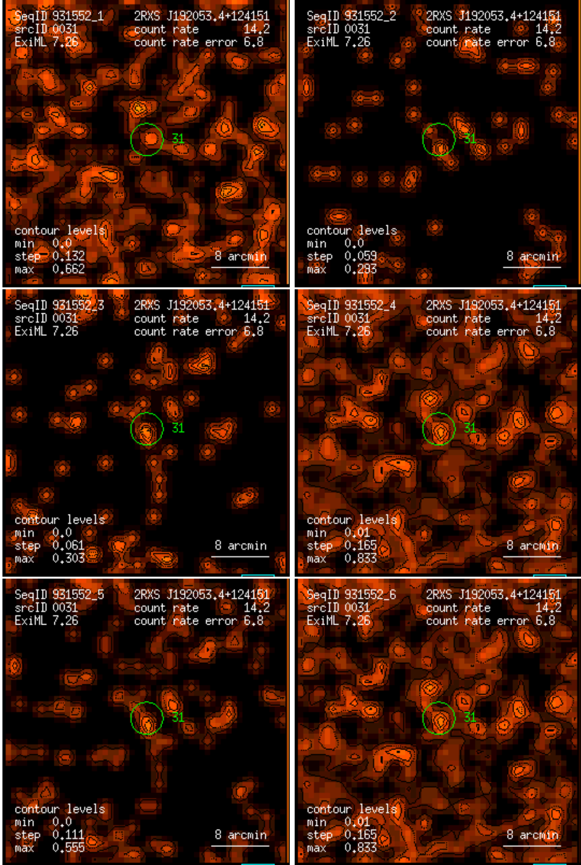
Figure 31: RASS 931552: detection 0031: band rate images, Gaussian filter: (1) PSPC channels 11 – 41, (2) 52 – 90, (3) 91 – 201, (4) 11 – 235, (5) 52 – 201, (6) 11 – 201. Broad band rates in counts/ks. Band rate contour levels in counts/ks/arcmin 2 .
