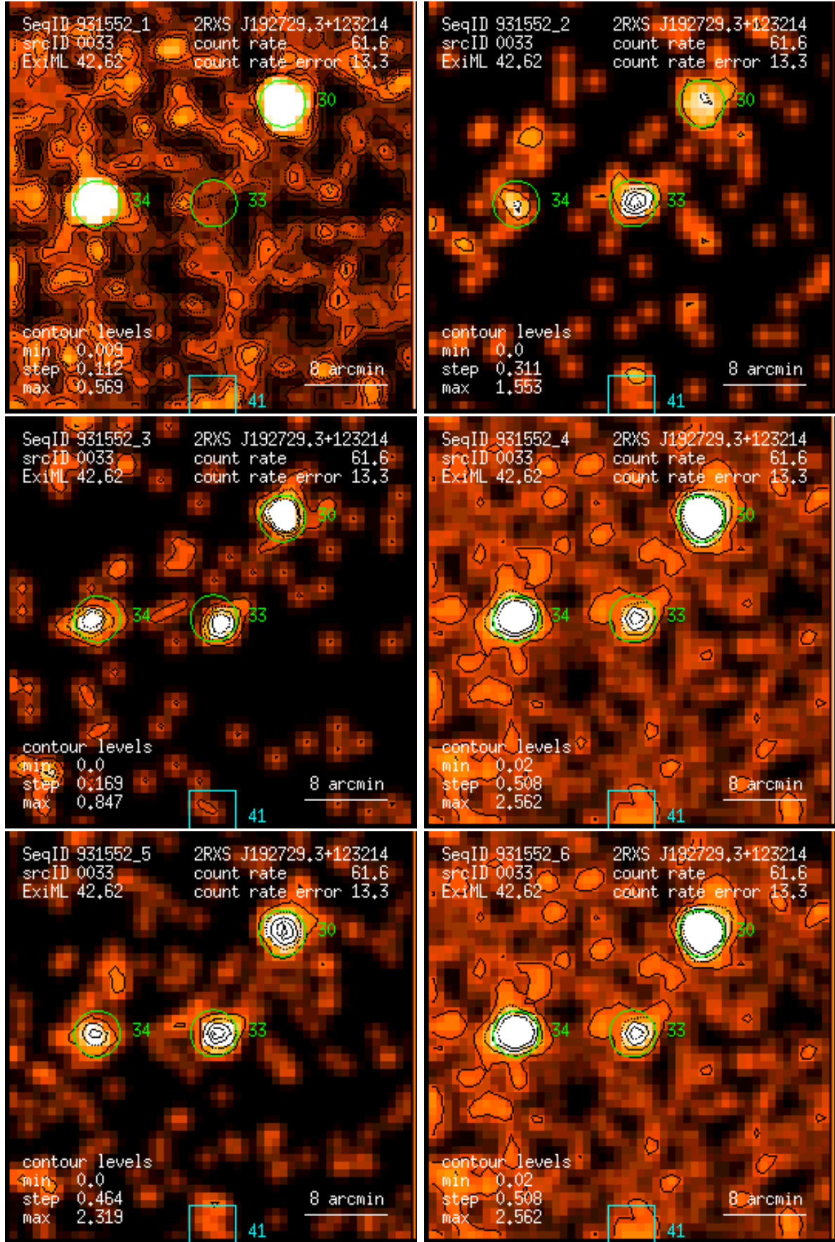
Figure 33: RASS 931552: detection 0033: band rate images, Gaussian filter: (1) PSPC channels 11 – 41, (2) 52 – 90, (3) 91 – 201, (4) 11 – 235, (5) 52 – 201, (6) 11 – 201. Broad band rates in counts/ks. Band rate contour levels in counts/ks/arcmin 2 .
