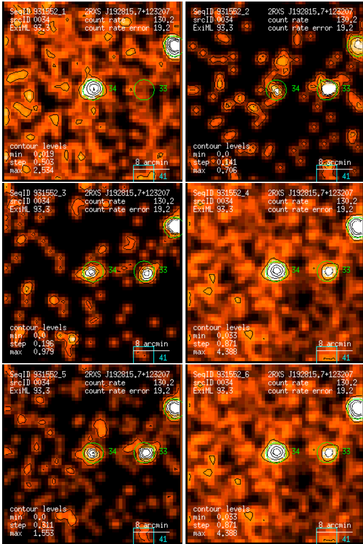
Figure 34: RASS 931552: detection 0034: band rate images, Gaussian filter: (1) PSPC channels 11 – 41, (2) 52 – 90, (3) 91 – 201, (4) 11 – 235, (5) 52 – 201, (6) 11 – 201. Broad band rates in counts/ks. Band rate contour levels in counts/ks/arcmin 2 .
