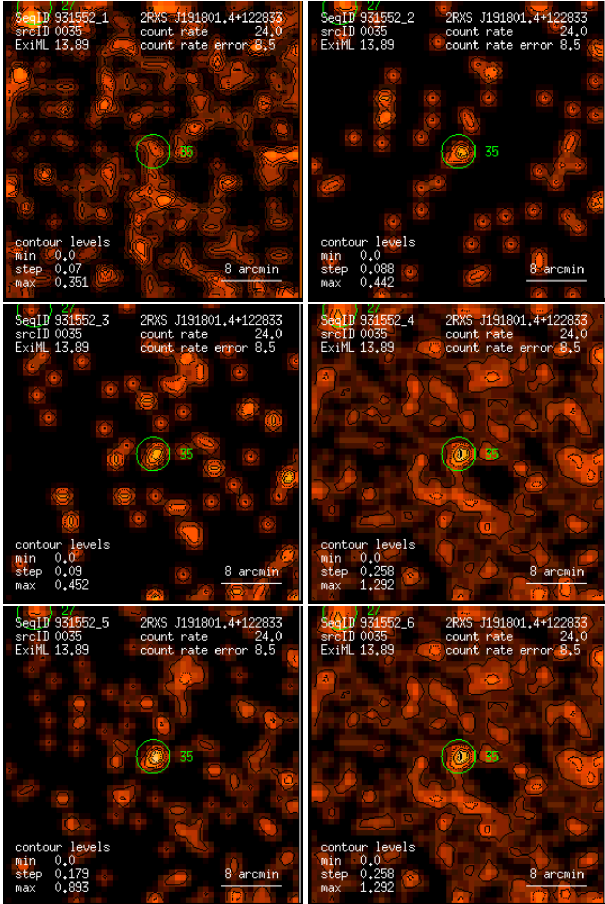
Figure 35: RASS 931552: detection 0035: band rate images, Gaussian filter: (1) PSPC channels 11 – 41, (2) 52 – 90, (3) 91 – 201, (4) 11 – 235, (5) 52 – 201, (6) 11 – 201. Broad band rates in counts/ks. Band rate contour levels in counts/ks/arcmin 2 .
