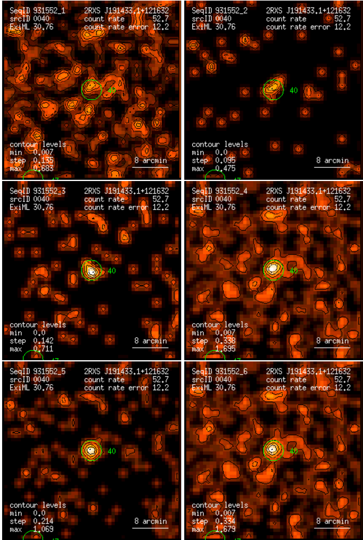
Figure 40: RASS 931552: detection 0040: band rate images, Gaussian filter: (1) PSPC channels 11 – 41, (2) 52 – 90, (3) 91 – 201, (4) 11 – 235, (5) 52 – 201, (6) 11 – 201. Broad band rates in counts/ks. Band rate contour levels in counts/ks/arcmin 2 .
