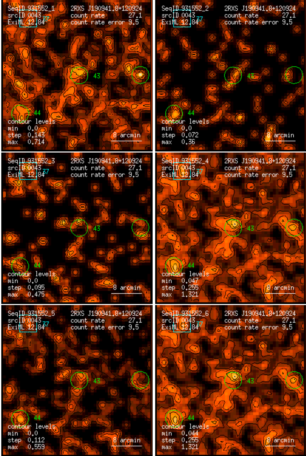
Figure 43: RASS 931552: detection 0043: band rate images, Gaussian filter: (1) PSPC channels 11 – 41, (2) 52 – 90, (3) 91 – 201, (4) 11 – 235, (5) 52 – 201, (6) 11 – 201. Broad band rates in counts/ks. Band rate contour levels in counts/ks/arcmin 2 .
