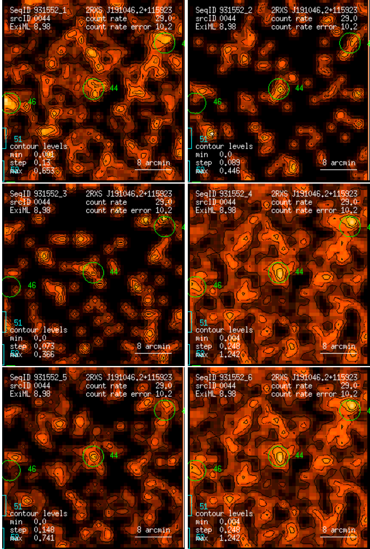
Figure 44: RASS 931552: detection 0044: band rate images, Gaussian filter: (1) PSPC channels 11 – 41, (2) 52 – 90, (3) 91 – 201, (4) 11 – 235, (5) 52 – 201, (6) 11 – 201. Broad band rates in counts/ks. Band rate contour levels in counts/ks/arcmin 2 .
