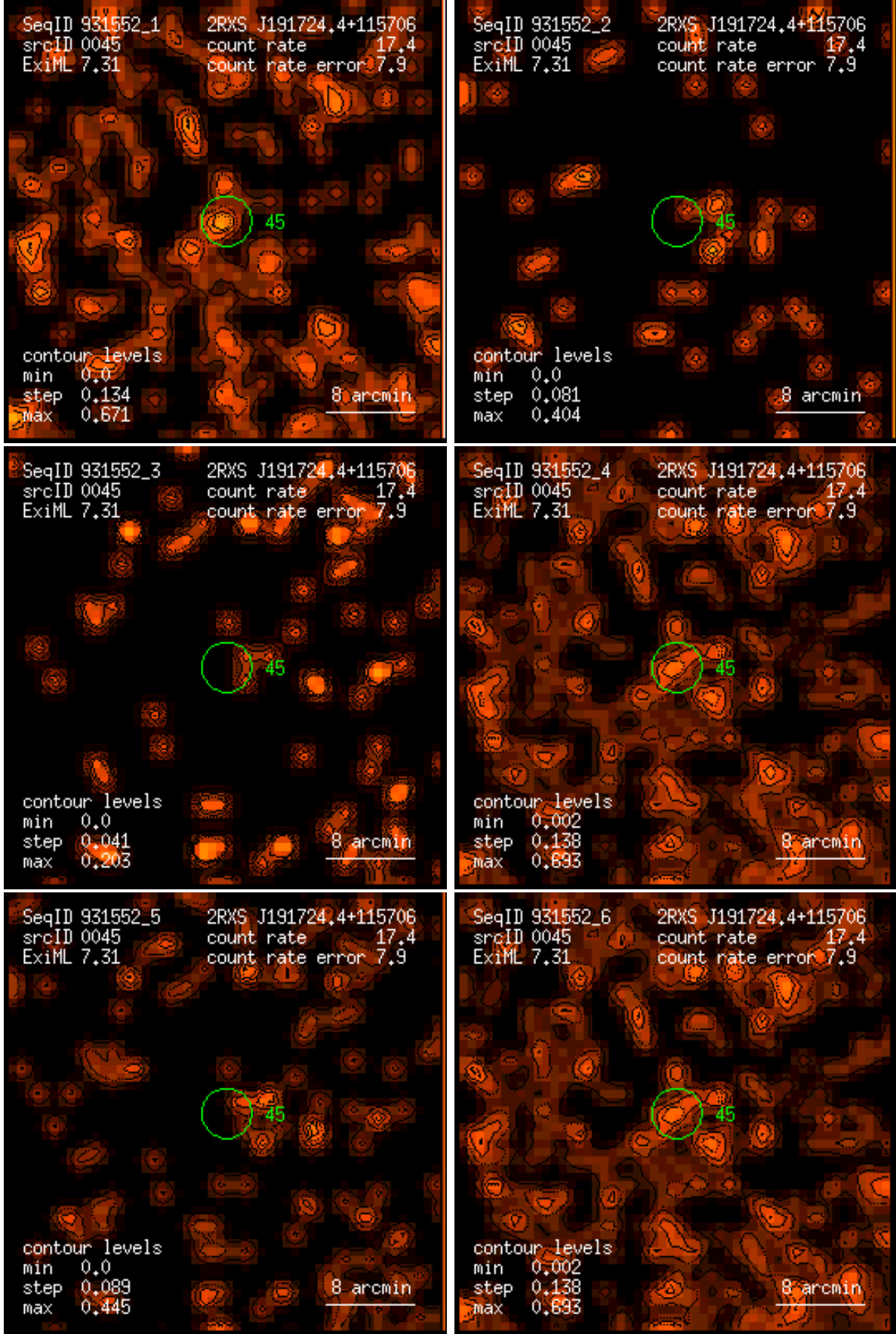
Figure 45: RASS 931552: detection 0045: band rate images, Gaussian filter: (1) PSPC channels 11 – 41, (2) 52 – 90, (3) 91 – 201, (4) 11 – 235, (5) 52 – 201, (6) 11 – 201. Broad band rates in counts/ks. Band rate contour levels in counts/ks/arcmin 2 .
