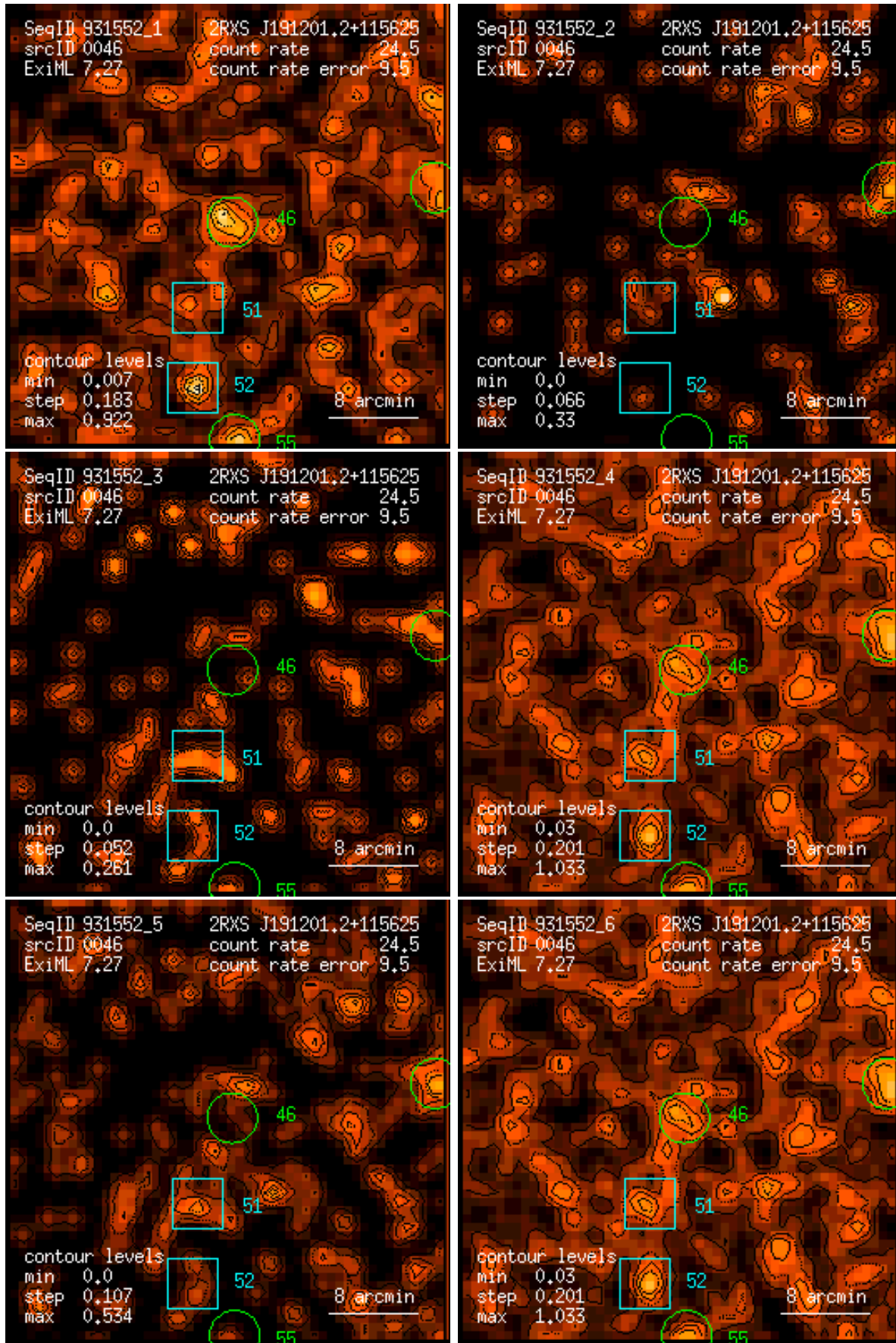
Figure 46: RASS 931552: detection 0046: band rate images, Gaussian filter: (1) PSPC channels 11 – 41, (2) 52 – 90, (3) 91 – 201, (4) 11 – 235, (5) 52 – 201, (6) 11 – 201. Broad band rates in counts/ks. Band rate contour levels in counts/ks/arcmin 2 .
