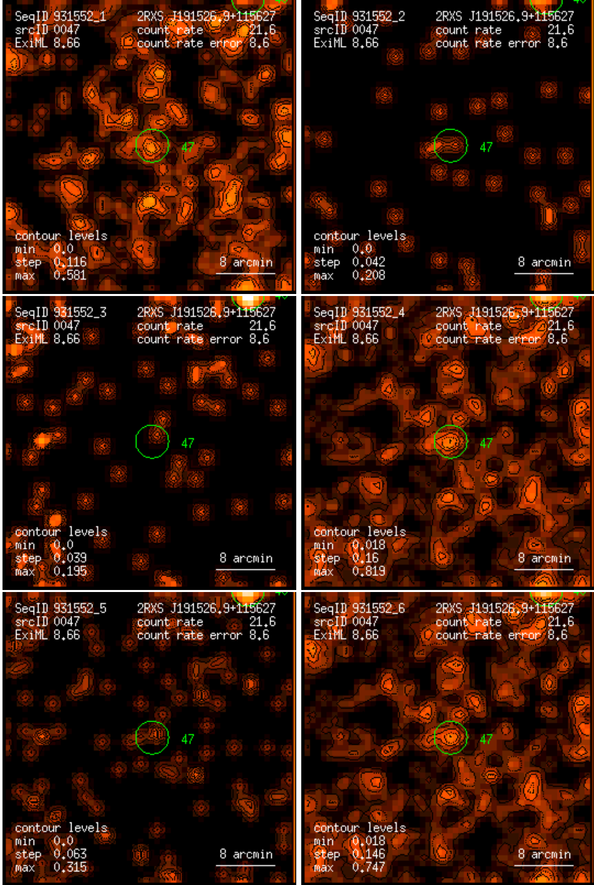
Figure 47: RASS 931552: detection 0047: band rate images, Gaussian filter: (1) PSPC channels 11 – 41, (2) 52 – 90, (3) 91 – 201, (4) 11 – 235, (5) 52 – 201, (6) 11 – 201. Broad band rates in counts/ks. Band rate contour levels in counts/ks/arcmin 2 .
