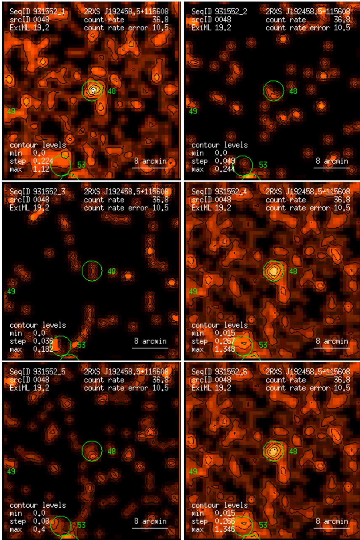
Figure 48: RASS 931552: detection 0048: band rate images, Gaussian filter: (1) PSPC channels 11 – 41, (2) 52 – 90, (3) 91 – 201, (4) 11 – 235, (5) 52 – 201, (6) 11 – 201. Broad band rates in counts/ks. Band rate contour levels in counts/ks/arcmin 2 .
