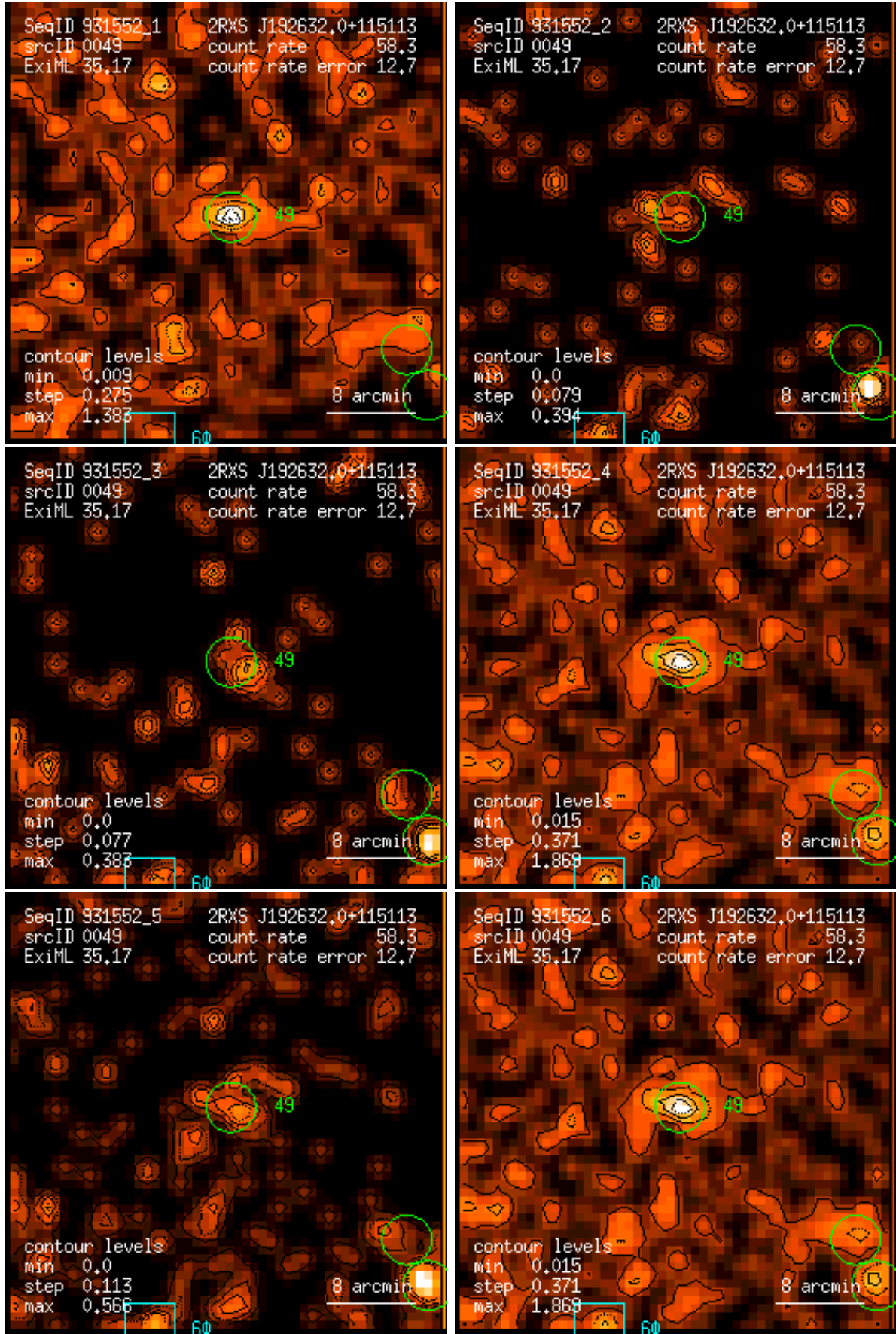
Figure 49: RASS 931552: detection 0049: band rate images, Gaussian filter: (1) PSPC channels 11 – 41, (2) 52 – 90, (3) 91 – 201, (4) 11 – 235, (5) 52 – 201, (6) 11 – 201. Broad band rates in counts/ks. Band rate contour levels in counts/ks/arcmin 2 .
