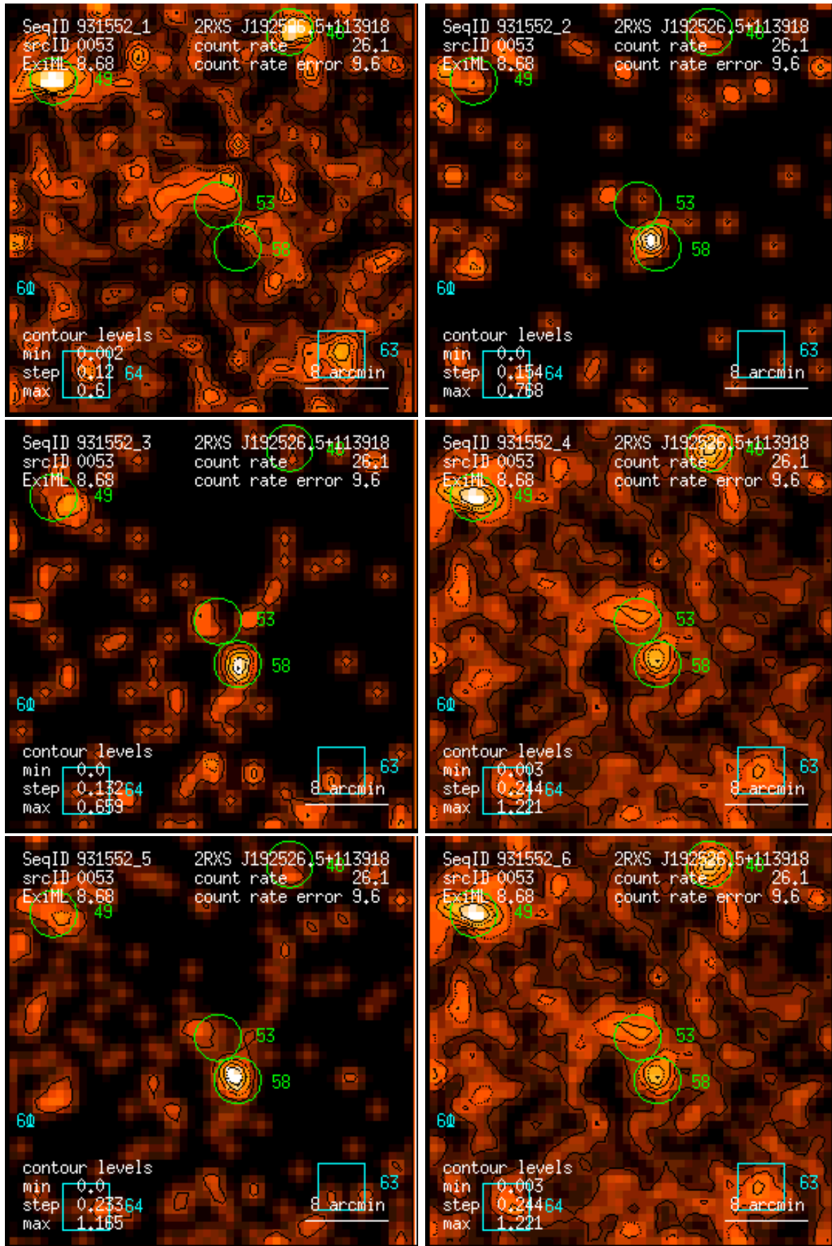
Figure 53: RASS 931552: detection 0053: band rate images, Gaussian filter: (1) PSPC channels 11 – 41, (2) 52 – 90, (3) 91 – 201, (4) 11 – 235, (5) 52 – 201, (6) 11 – 201. Broad band rates in counts/ks. Band rate contour levels in counts/ks/arcmin 2 .
