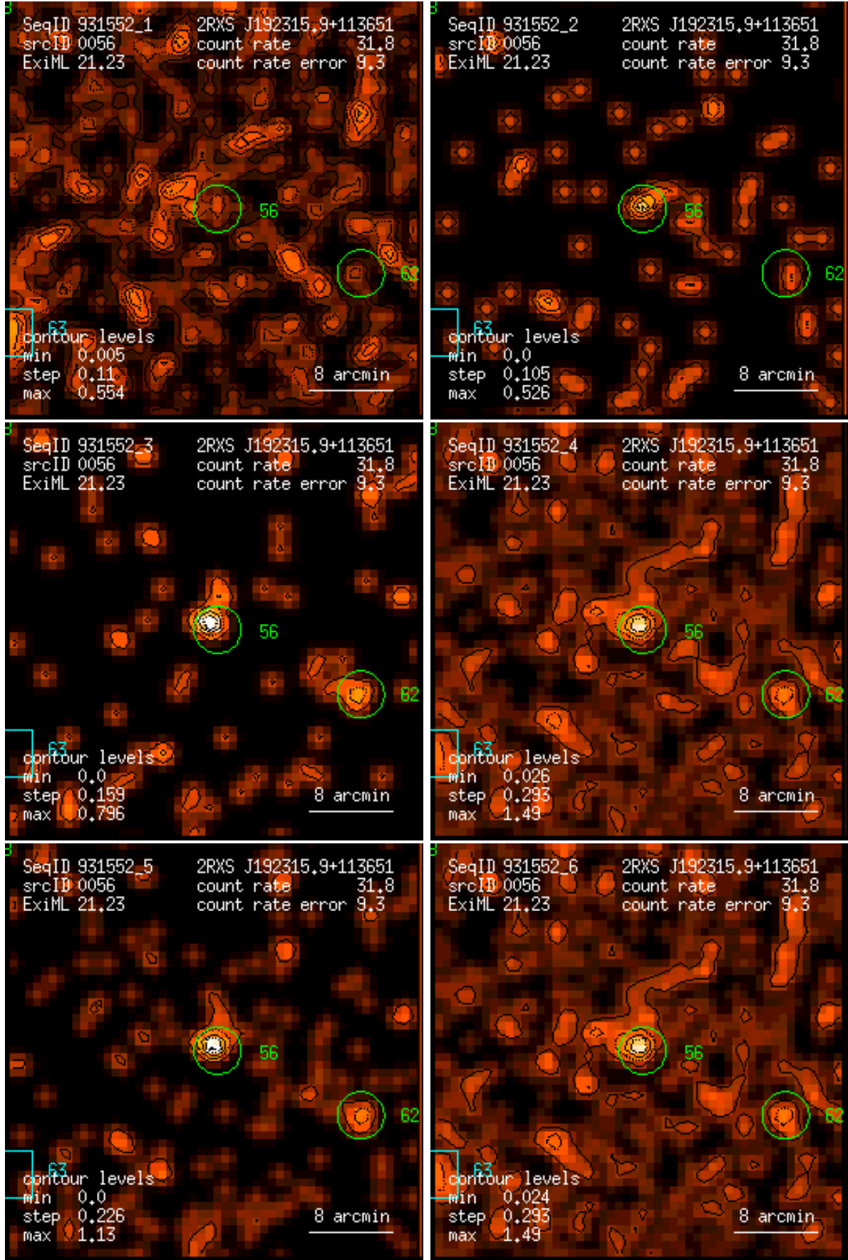
Figure 56: RASS 931552: detection 0056: band rate images, Gaussian filter: (1) PSPC channels 11 – 41, (2) 52 – 90, (3) 91 – 201, (4) 11 – 235, (5) 52 – 201, (6) 11 – 201. Broad band rates in counts/ks. Band rate contour levels in counts/ks/arcmin 2 .
