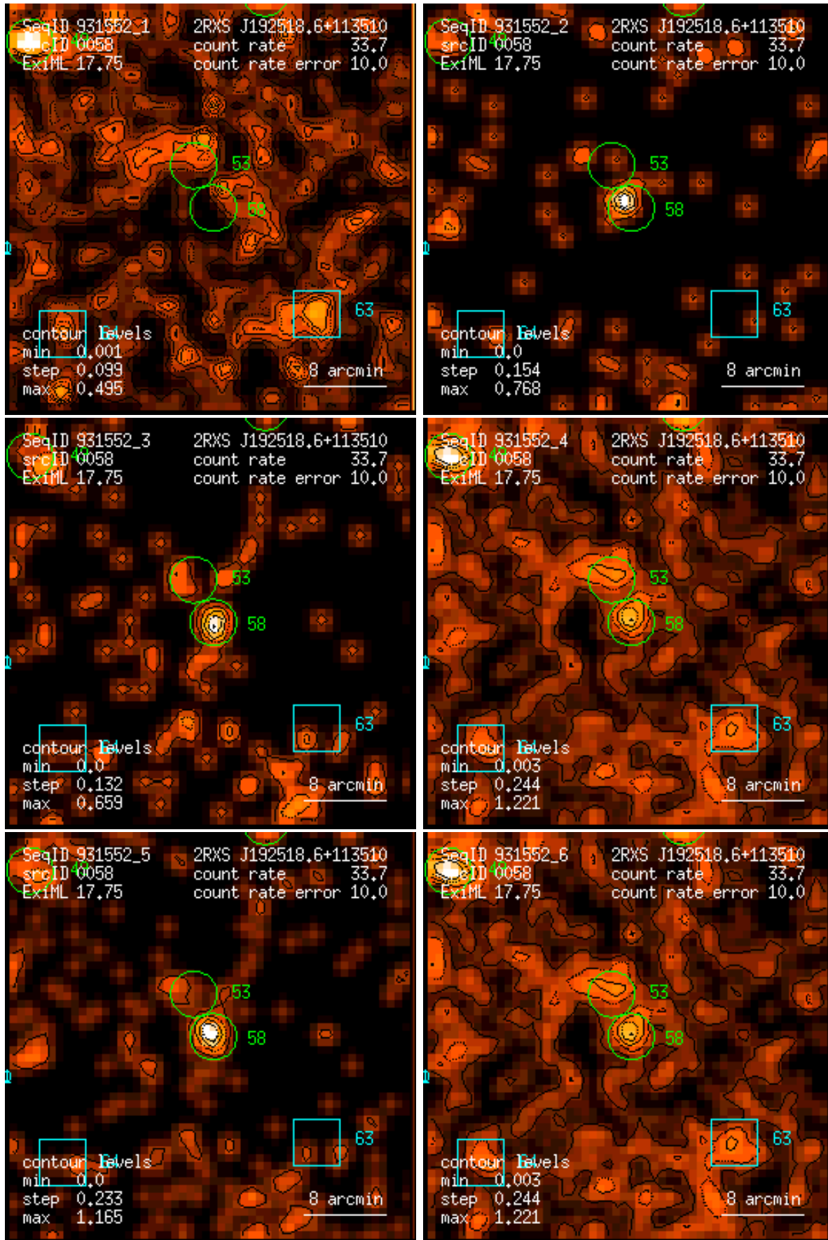
Figure 58: RASS 931552: detection 0058: band rate images, Gaussian filter: (1) PSPC channels 11 – 41, (2) 52 – 90, (3) 91 – 201, (4) 11 – 235, (5) 52 – 201, (6) 11 – 201. Broad band rates in counts/ks. Band rate contour levels in counts/ks/arcmin 2 .
