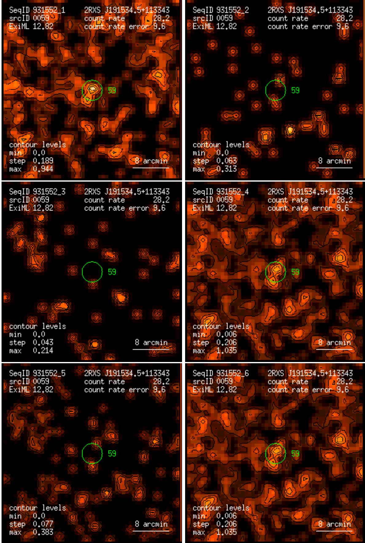
Figure 59: RASS 931552: detection 0059: band rate images, Gaussian filter: (1) PSPC channels 11 – 41, (2) 52 – 90, (3) 91 – 201, (4) 11 – 235, (5) 52 – 201, (6) 11 – 201. Broad band rates in counts/ks. Band rate contour levels in counts/ks/arcmin 2 .
