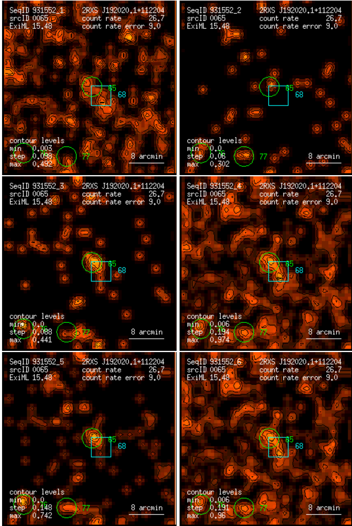
Figure 65: RASS 931552: detection 0065: band rate images, Gaussian filter: (1) PSPC channels 11 – 41, (2) 52 – 90, (3) 91 – 201, (4) 11 – 235, (5) 52 – 201, (6) 11 – 201. Broad band rates in counts/ks. Band rate contour levels in counts/ks/arcmin 2 .
