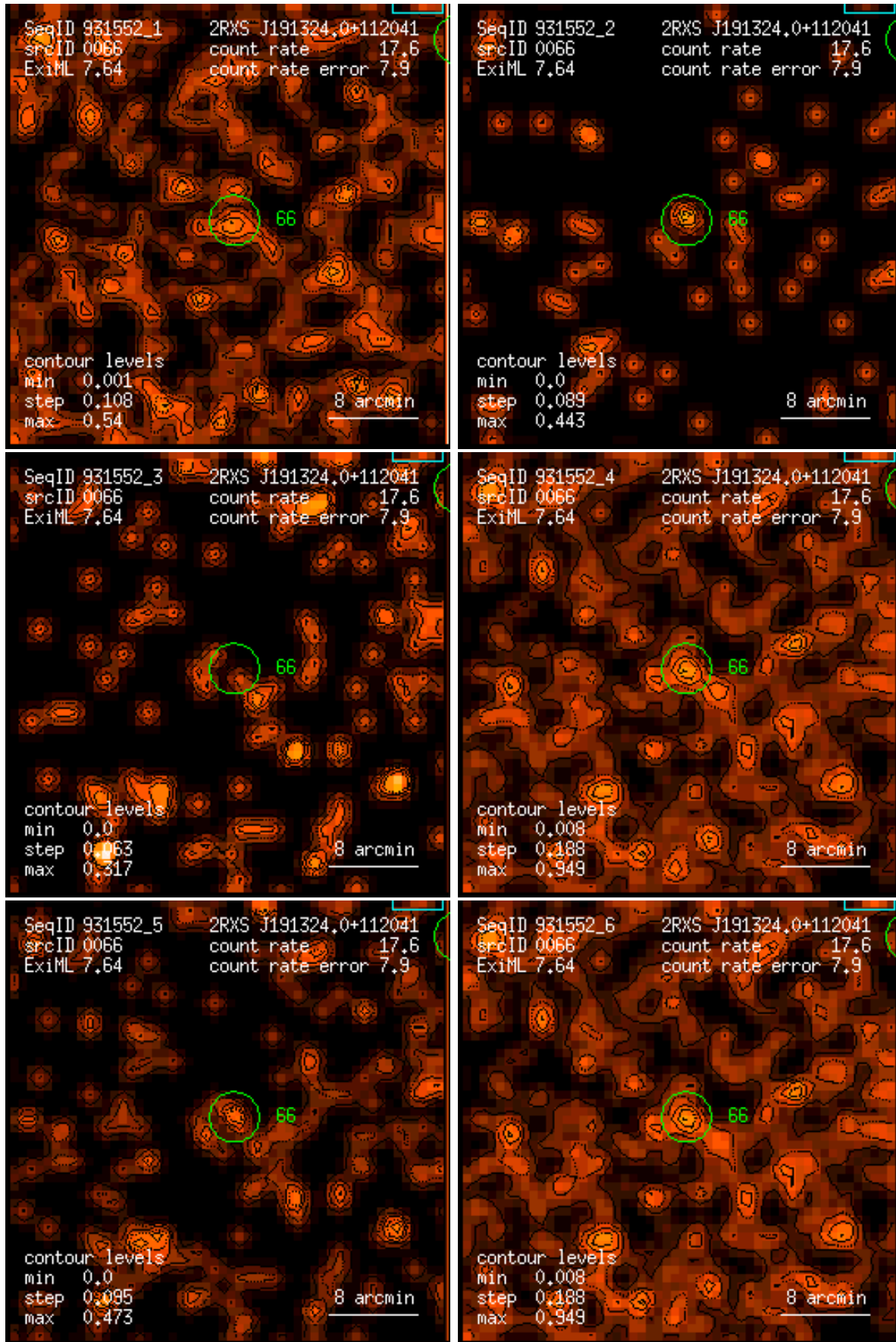
Figure 66: RASS 931552: detection 0066: band rate images, Gaussian filter: (1) PSPC channels 11 – 41, (2) 52 – 90, (3) 91 – 201, (4) 11 – 235, (5) 52 – 201, (6) 11 – 201. Broad band rates in counts/ks. Band rate contour levels in counts/ks/arcmin 2 .
