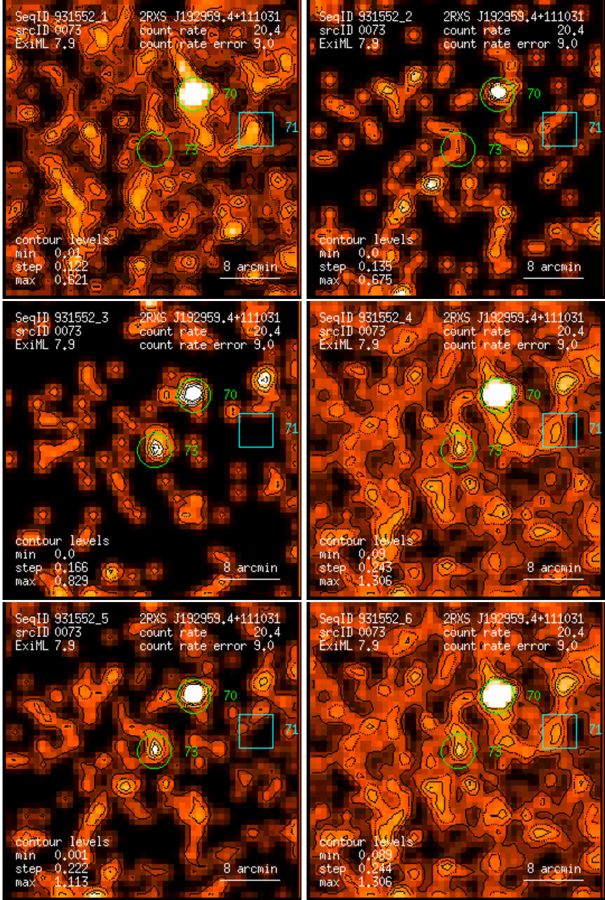
Figure 73: RASS 931552: detection 0073: band rate images, Gaussian filter: (1) PSPC channels 11 – 41, (2) 52 – 90, (3) 91 – 201, (4) 11 – 235, (5) 52 – 201, (6) 11 – 201. Broad band rates in counts/ks. Band rate contour levels in counts/ks/arcmin 2 .
