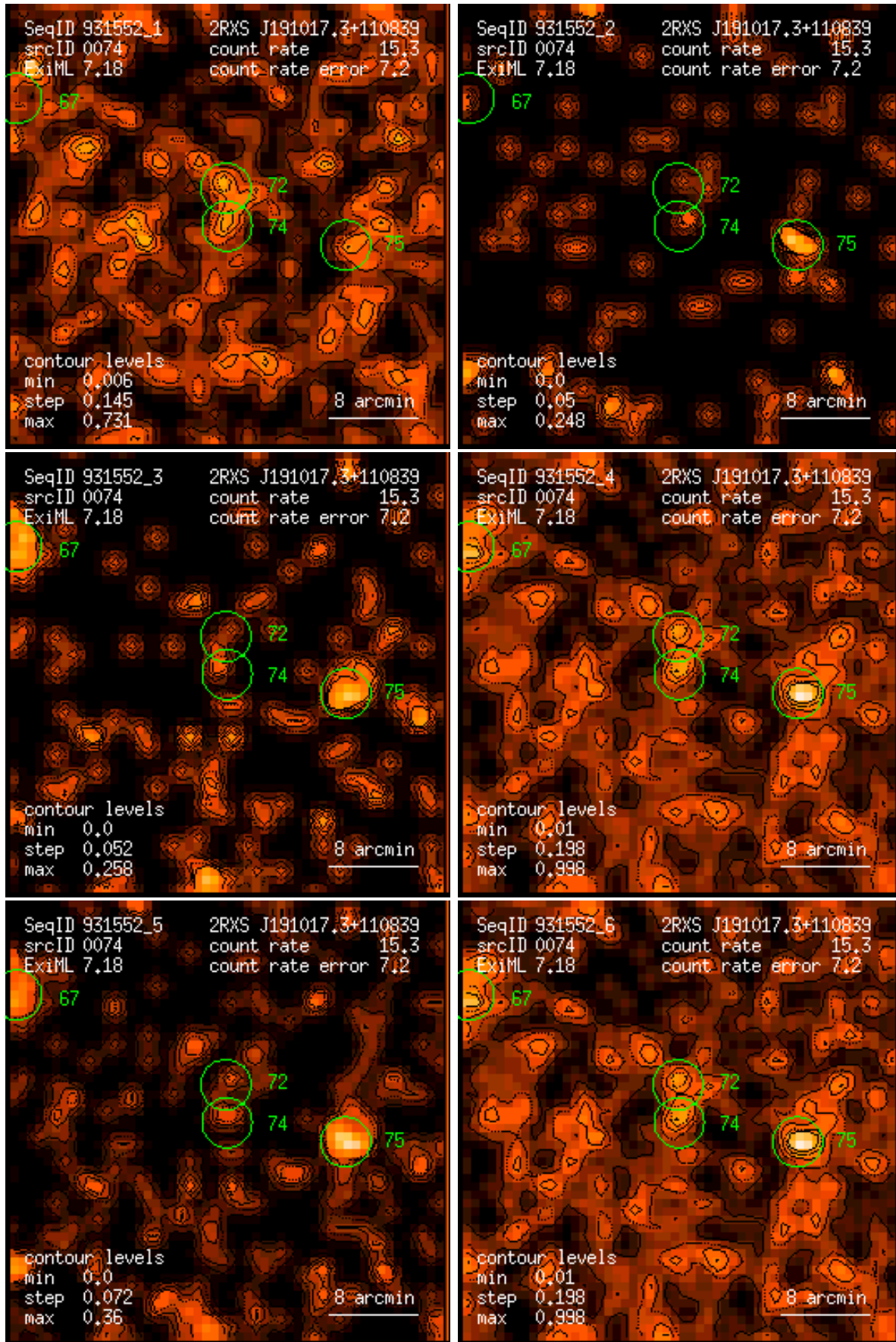
Figure 74: RASS 931552: detection 0074: band rate images, Gaussian filter: (1) PSPC channels 11 – 41, (2) 52 – 90, (3) 91 – 201, (4) 11 – 235, (5) 52 – 201, (6) 11 – 201. Broad band rates in counts/ks. Band rate contour levels in counts/ks/arcmin 2 .
