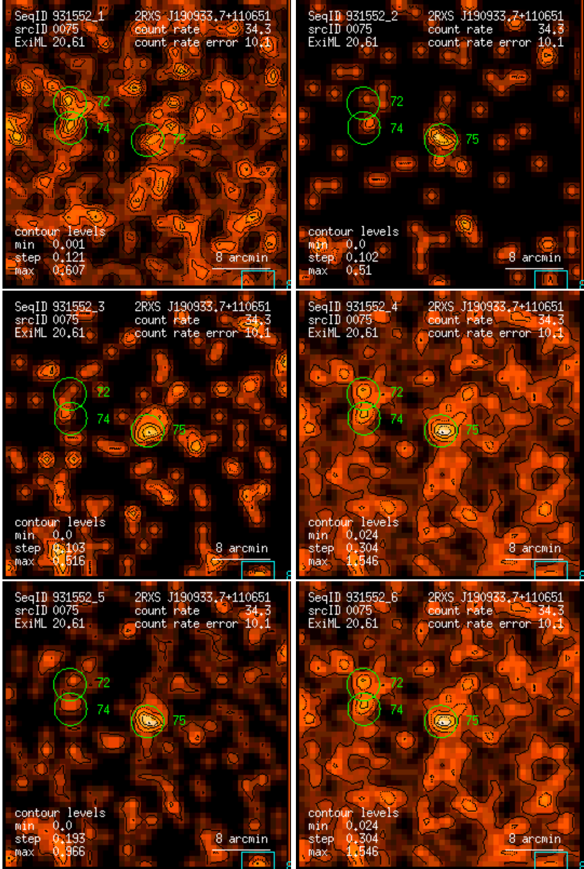
Figure 75: RASS 931552: detection 0075: band rate images, Gaussian filter: (1) PSPC channels 11 – 41, (2) 52 – 90, (3) 91 – 201, (4) 11 – 235, (5) 52 – 201, (6) 11 – 201. Broad band rates in counts/ks. Band rate contour levels in counts/ks/arcmin 2 .
