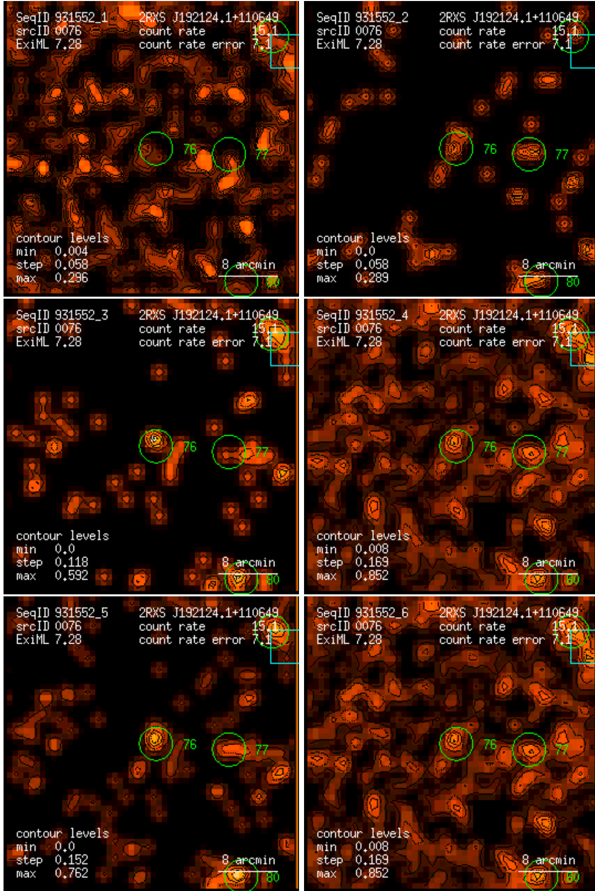
Figure 76: RASS 931552: detection 0076: band rate images, Gaussian filter: (1) PSPC channels 11 – 41, (2) 52 – 90, (3) 91 – 201, (4) 11 – 235, (5) 52 – 201, (6) 11 – 201. Broad band rates in counts/ks. Band rate contour levels in counts/ks/arcmin 2 .
