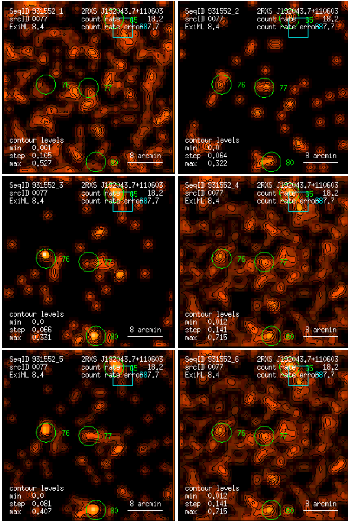
Figure 77: RASS 931552: detection 0077: band rate images, Gaussian filter: (1) PSPC channels 11 – 41, (2) 52 – 90, (3) 91 – 201, (4) 11 – 235, (5) 52 – 201, (6) 11 – 201. Broad band rates in counts/ks. Band rate contour levels in counts/ks/arcmin 2 .
