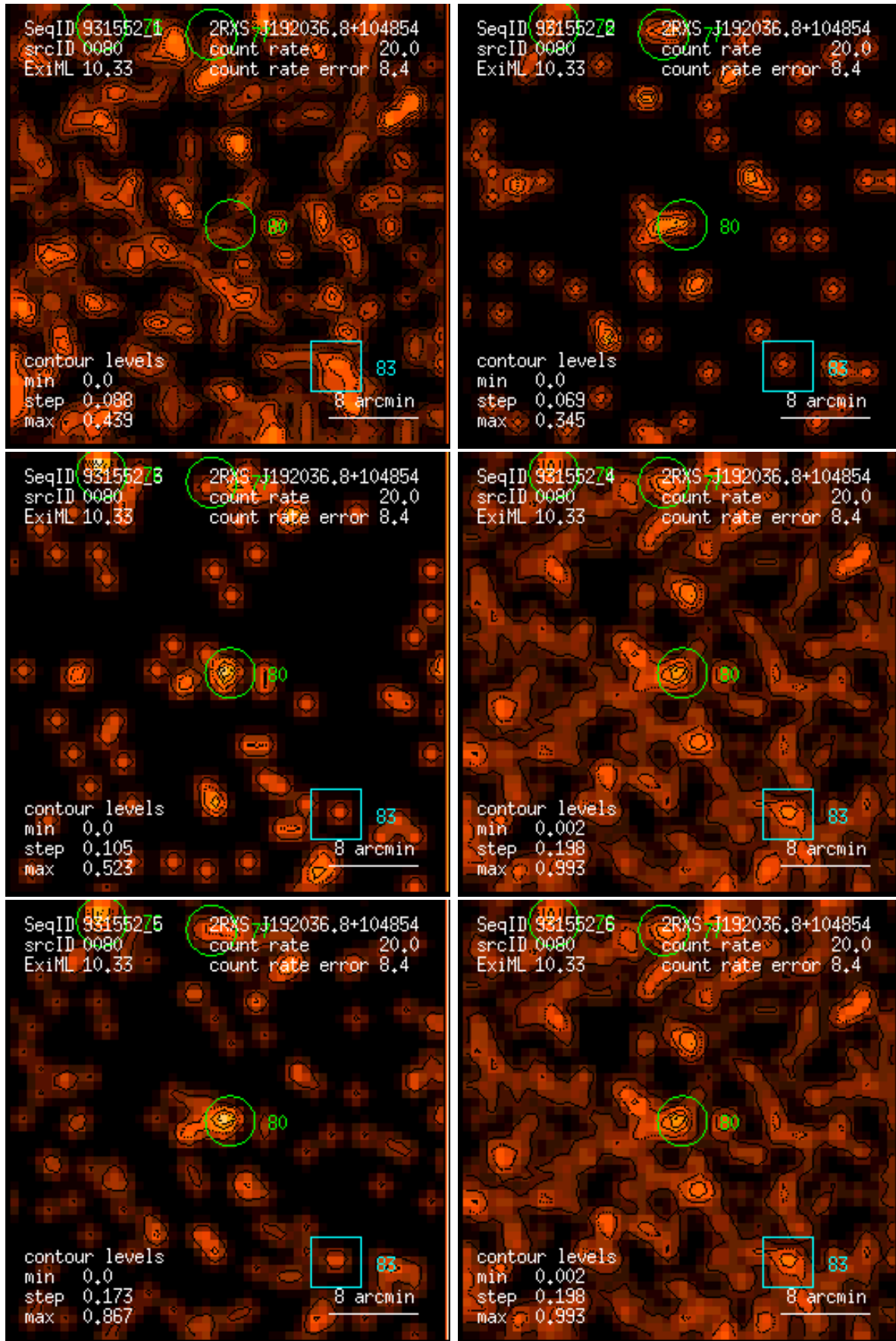
Figure 80: RASS 931552: detection 0080: band rate images, Gaussian filter: (1) PSPC channels 11 – 41, (2) 52 – 90, (3) 91 – 201, (4) 11 – 235, (5) 52 – 201, (6) 11 – 201. Broad band rates in counts/ks. Band rate contour levels in counts/ks/arcmin 2 .
