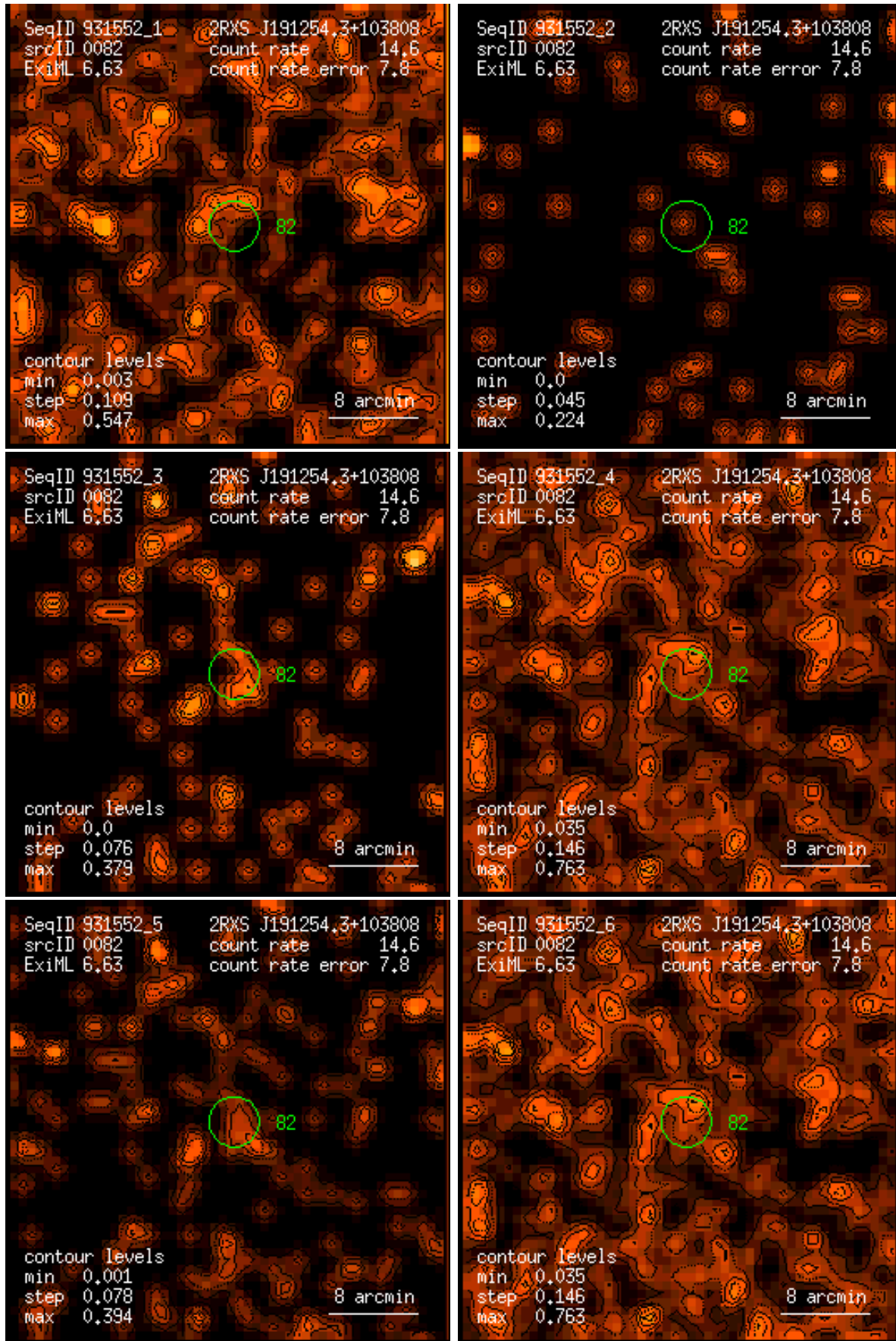
Figure 82: RASS 931552: detection 0082: band rate images, Gaussian filter: (1) PSPC channels 11 – 41, (2) 52 – 90, (3) 91 – 201, (4) 11 – 235, (5) 52 – 201, (6) 11 – 201. Broad band rates in counts/ks. Band rate contour levels in counts/ks/arcmin 2 .
