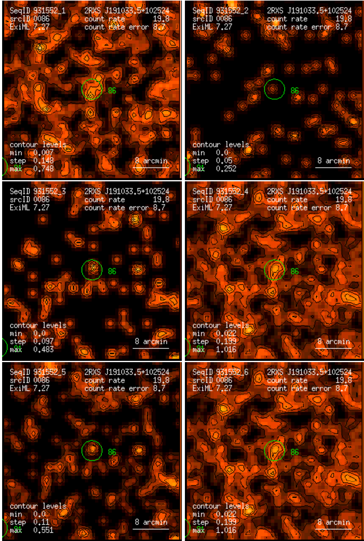
Figure 86: RASS 931552: detection 0086: band rate images, Gaussian filter: (1) PSPC channels 11 – 41, (2) 52 – 90, (3) 91 – 201, (4) 11 – 235, (5) 52 – 201, (6) 11 – 201. Broad band rates in counts/ks. Band rate contour levels in counts/ks/arcmin 2 .
