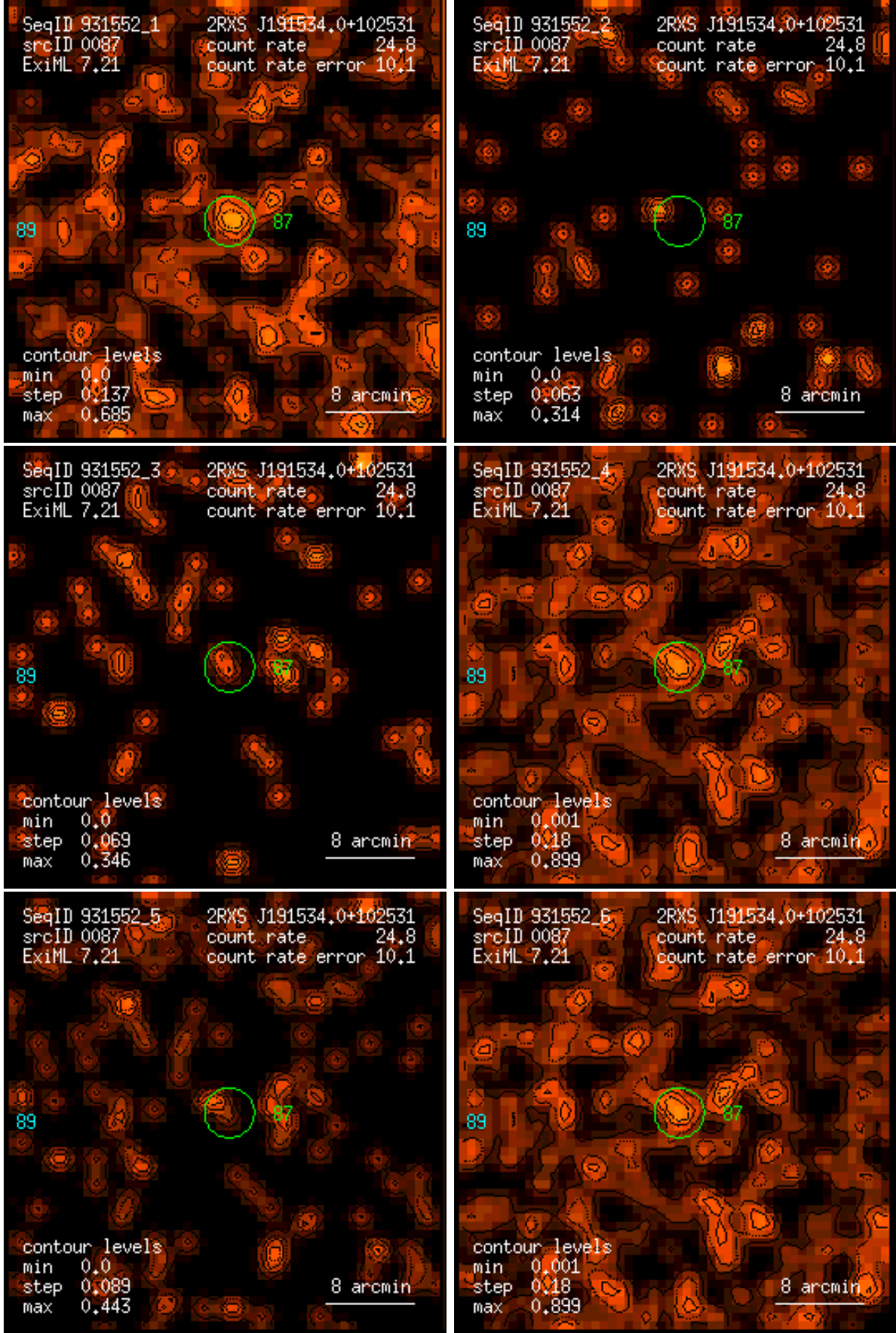
Figure 87: RASS 931552: detection 0087: band rate images, Gaussian filter: (1) PSPC channels 11 – 41, (2) 52 – 90, (3) 91 – 201, (4) 11 – 235, (5) 52 – 201, (6) 11 – 201. Broad band rates in counts/ks. Band rate contour levels in counts/ks/arcmin 2 .
