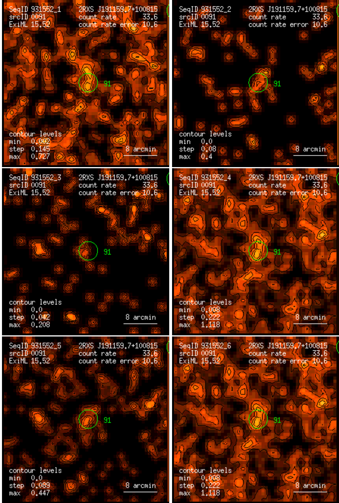
Figure 91: RASS 931552: detection 0091: band rate images, Gaussian filter: (1) PSPC channels 11 – 41, (2) 52 – 90, (3) 91 – 201, (4) 11 – 235, (5) 52 – 201, (6) 11 – 201. Broad band rates in counts/ks. Band rate contour levels in counts/ks/arcmin 2 .
