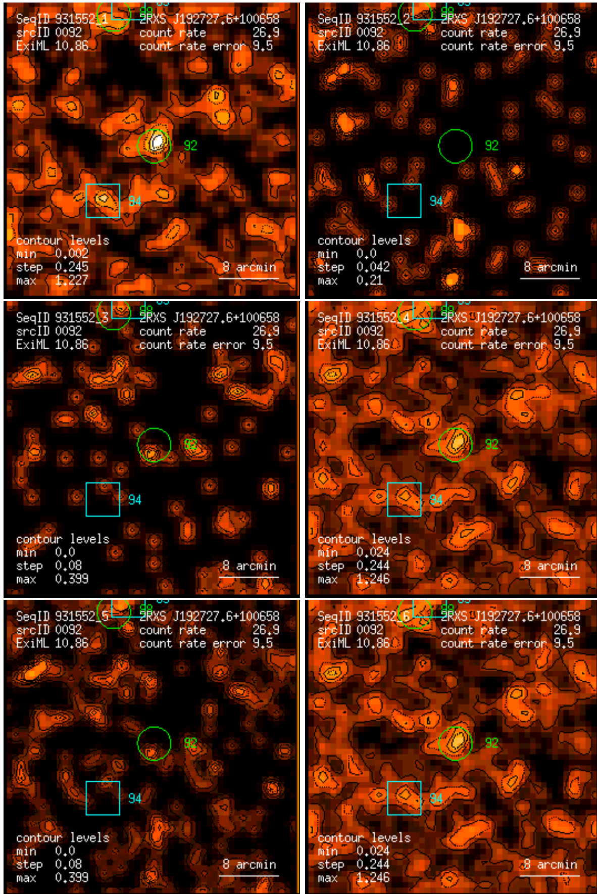
Figure 92: RASS 931552: detection 0092: band rate images, Gaussian filter: (1) PSPC channels 11 – 41, (2) 52 – 90, (3) 91 – 201, (4) 11 – 235, (5) 52 – 201, (6) 11 – 201. Broad band rates in counts/ks. Band rate contour levels in counts/ks/arcmin 2 .
