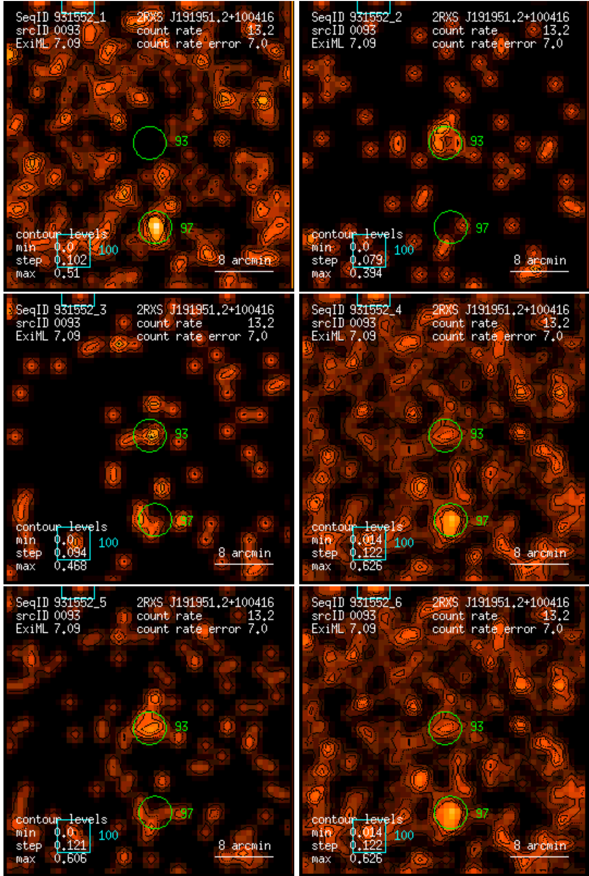
Figure 93: RASS 931552: detection 0093: band rate images, Gaussian filter: (1) PSPC channels 11 – 41, (2) 52 – 90, (3) 91 – 201, (4) 11 – 235, (5) 52 – 201, (6) 11 – 201. Broad band rates in counts/ks. Band rate contour levels in counts/ks/arcmin 2 .
