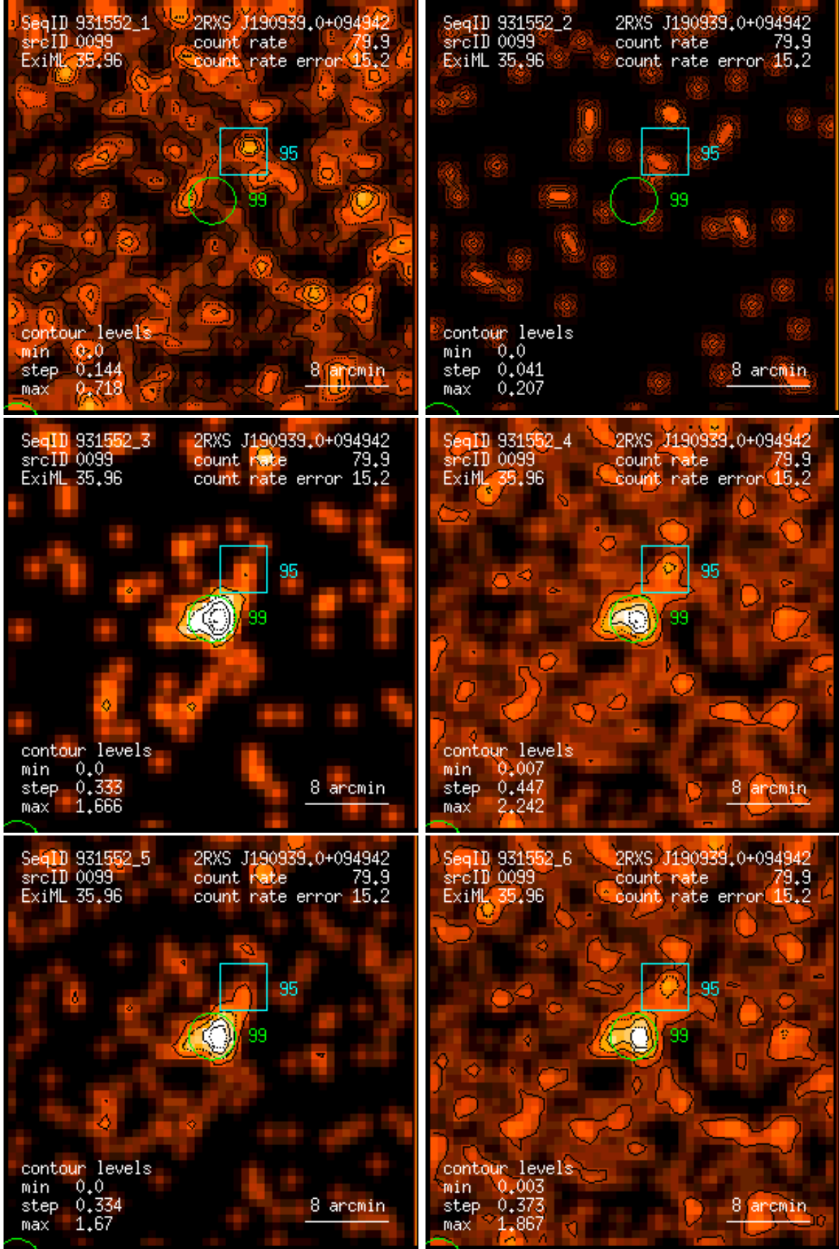
Figure 99: RASS 931552: detection 0099: band rate images, Gaussian filter: (1) PSPC channels 11 – 41, (2) 52 – 90, (3) 91 – 201, (4) 11 – 235, (5) 52 – 201, (6) 11 – 201. Broad band rates in counts/ks. Band rate contour levels in counts/ks/arcmin 2 .
