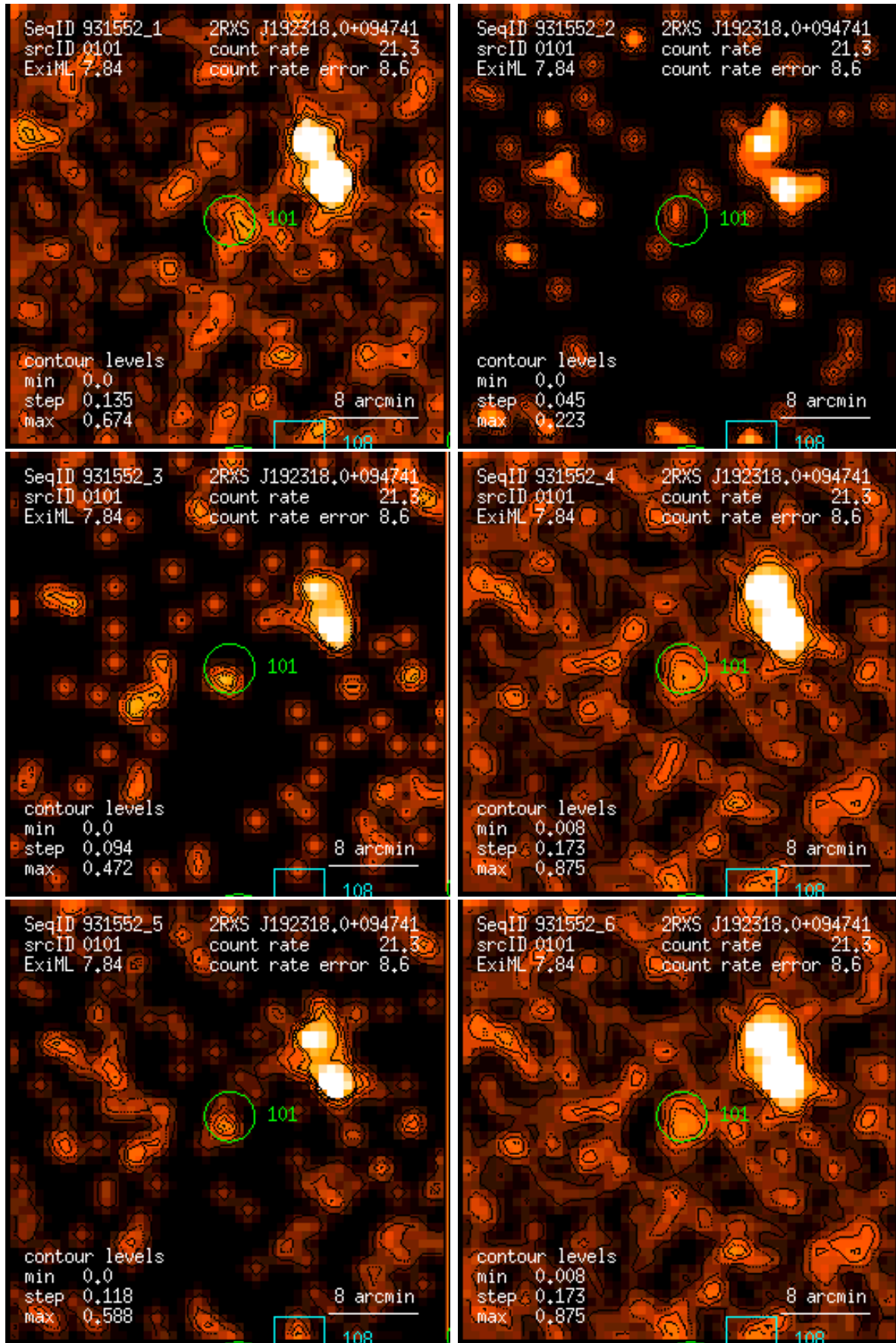
Figure 101: RASS 931552: detection 0101: band rate images, Gaussian filter: (1) PSPC channels 11 – 41, (2) 52 – 90, (3) 91 – 201, (4) 11 – 235, (5) 52 – 201, (6) 11 – 201. Broad band rates in counts/ks. Band rate contour levels in counts/ks/arcmin 2 .
