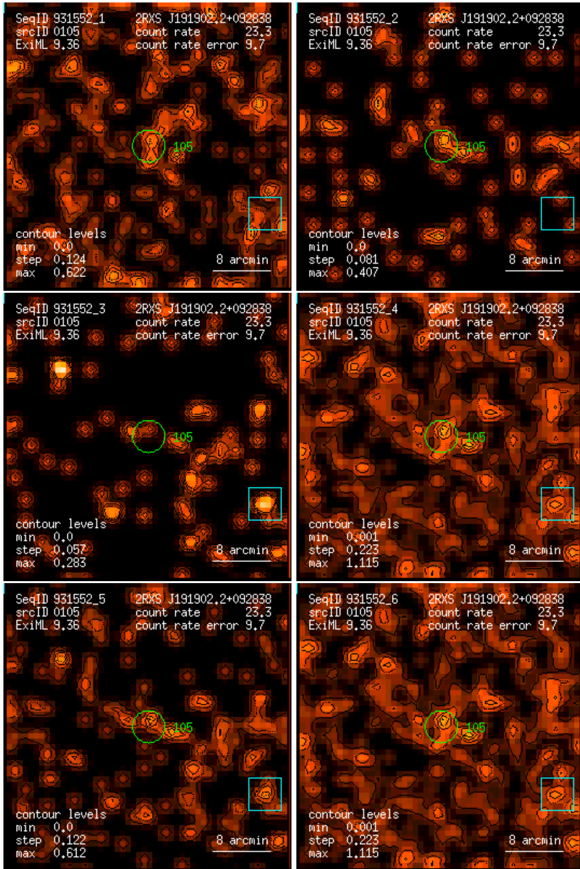
Figure 105: RASS 931552: detection 0105: band rate images, Gaussian filter: (1) PSPC channels 11 – 41, (2) 52 – 90, (3) 91 – 201, (4) 11 – 235, (5) 52 – 201, (6) 11 – 201. Broad band rates in counts/ks. Band rate contour levels in counts/ks/arcmin 2 .
