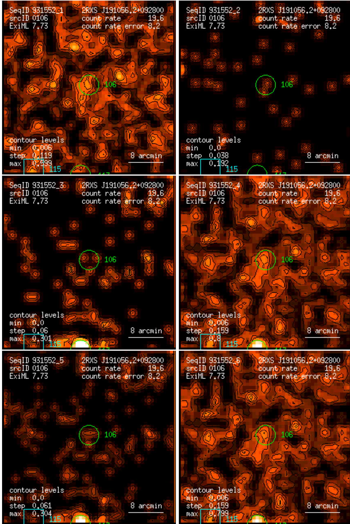
Figure 106: RASS 931552: detection 0106: band rate images, Gaussian filter: (1) PSPC channels 11 – 41, (2) 52 – 90, (3) 91 – 201, (4) 11 – 235, (5) 52 – 201, (6) 11 – 201. Broad band rates in counts/ks. Band rate contour levels in counts/ks/arcmin 2 .
