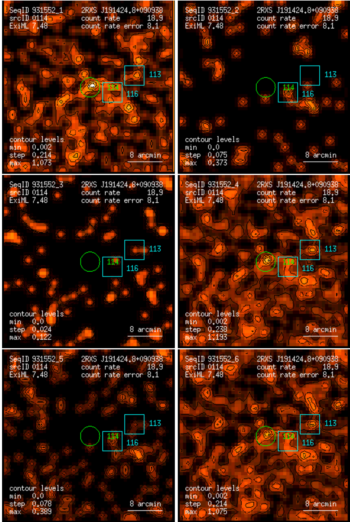
Figure 114: RASS 931552: detection 0114: band rate images, Gaussian filter: (1) PSPC channels 11 – 41, (2) 52 – 90, (3) 91 – 201, (4) 11 – 235, (5) 52 – 201, (6) 11 – 201. Broad band rates in counts/ks. Band rate contour levels in counts/ks/arcmin 2 .
