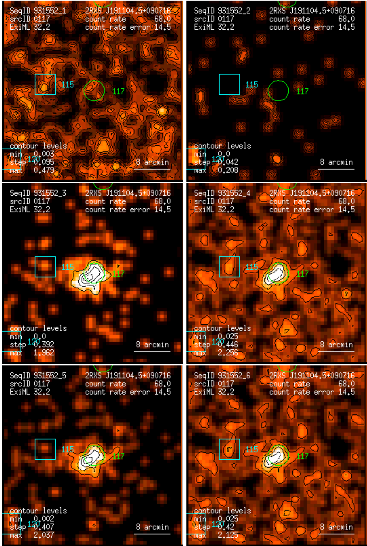
Figure 117: RASS 931552: detection 0117: band rate images, Gaussian filter: (1) PSPC channels 11 – 41, (2) 52 – 90, (3) 91 – 201, (4) 11 – 235, (5) 52 – 201, (6) 11 – 201. Broad band rates in counts/ks. Band rate contour levels in counts/ks/arcmin 2 .
