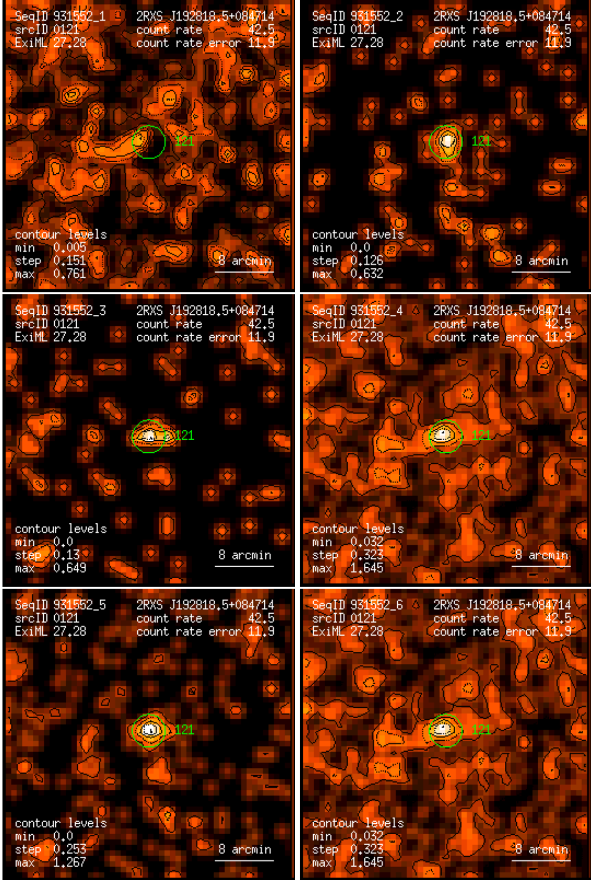
Figure 121: RASS 931552: detection 0121: band rate images, Gaussian filter: (1) PSPC channels 11 – 41, (2) 52 – 90, (3) 91 – 201, (4) 11 – 235, (5) 52 – 201, (6) 11 – 201. Broad band rates in counts/ks. Band rate contour levels in counts/ks/arcmin 2 .
