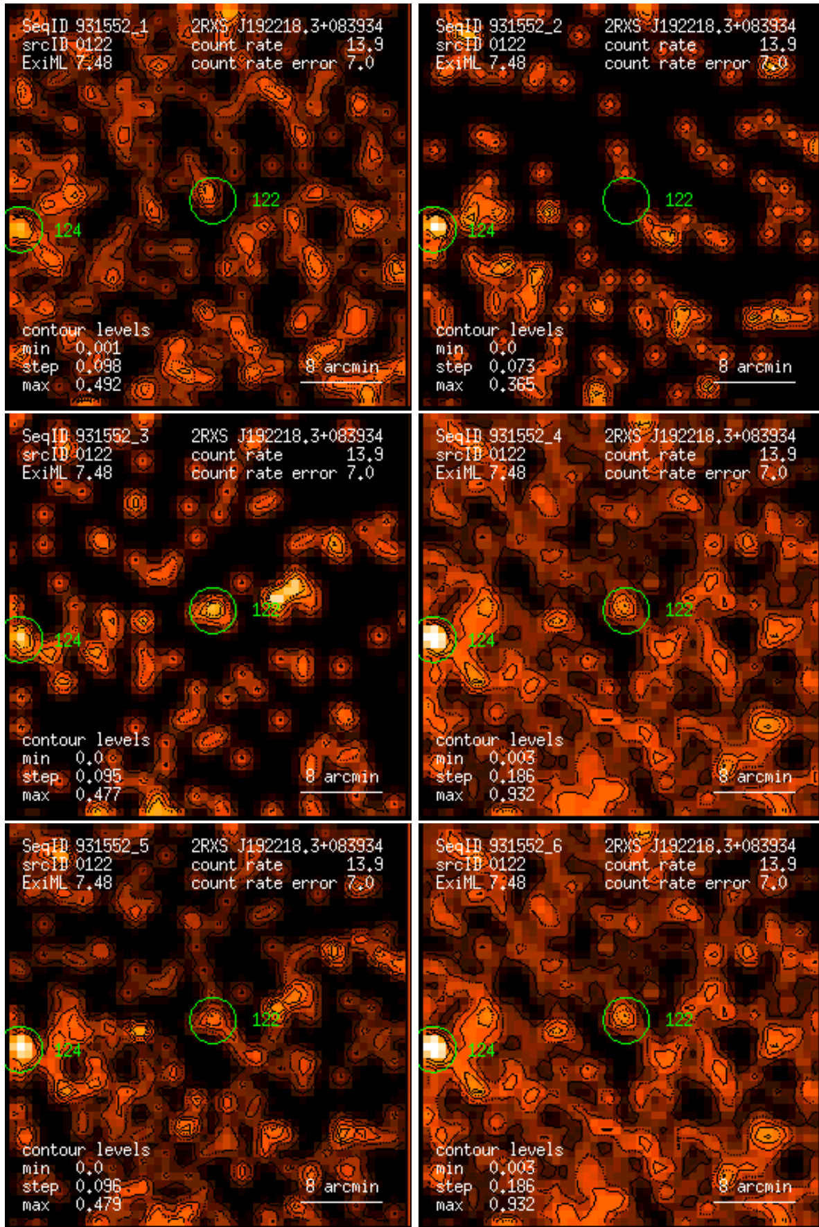
Figure 122: RASS 931552: detection 0122: band rate images, Gaussian filter: (1) PSPC channels 11 – 41, (2) 52 – 90, (3) 91 – 201, (4) 11 – 235, (5) 52 – 201, (6) 11 – 201. Broad band rates in counts/ks. Band rate contour levels in counts/ks/arcmin 2 .
