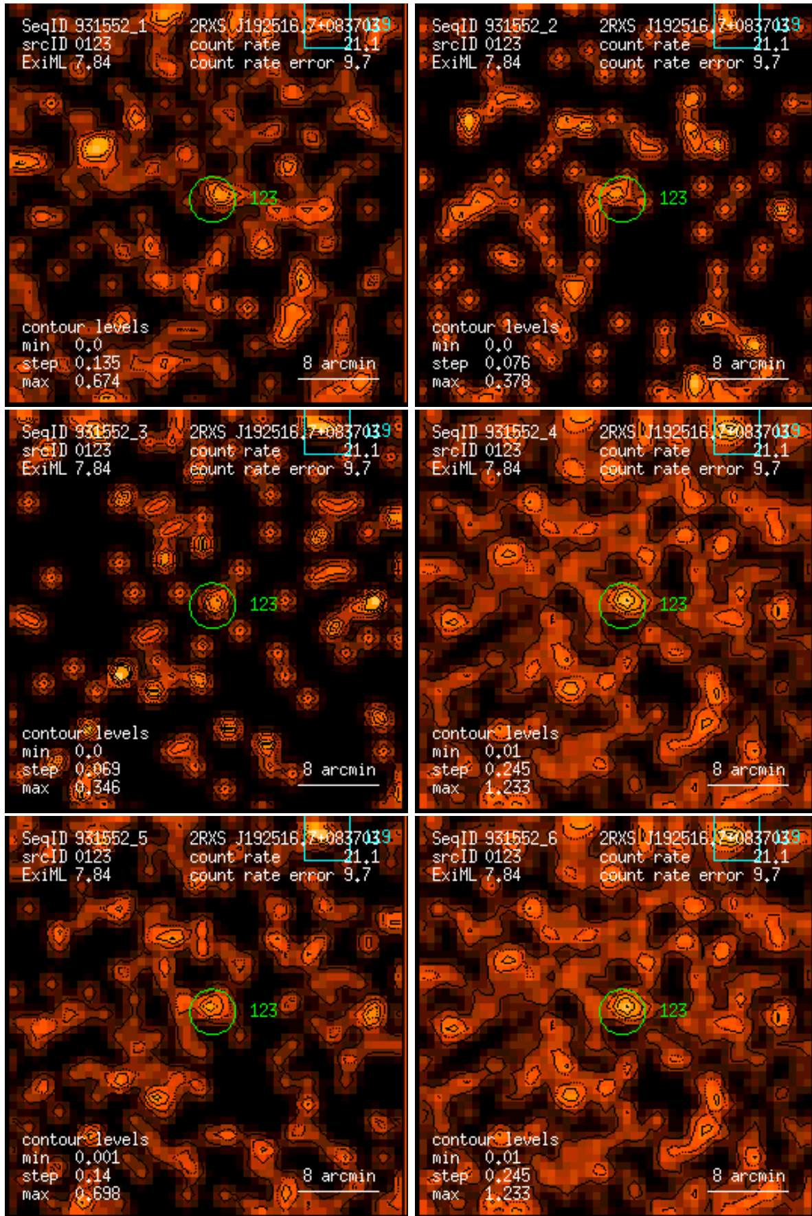
Figure 123: RASS 931552: detection 0123: band rate images, Gaussian filter: (1) PSPC channels 11 – 41, (2) 52 – 90, (3) 91 – 201, (4) 11 – 235, (5) 52 – 201, (6) 11 – 201. Broad band rates in counts/ks. Band rate contour levels in counts/ks/arcmin 2 .
