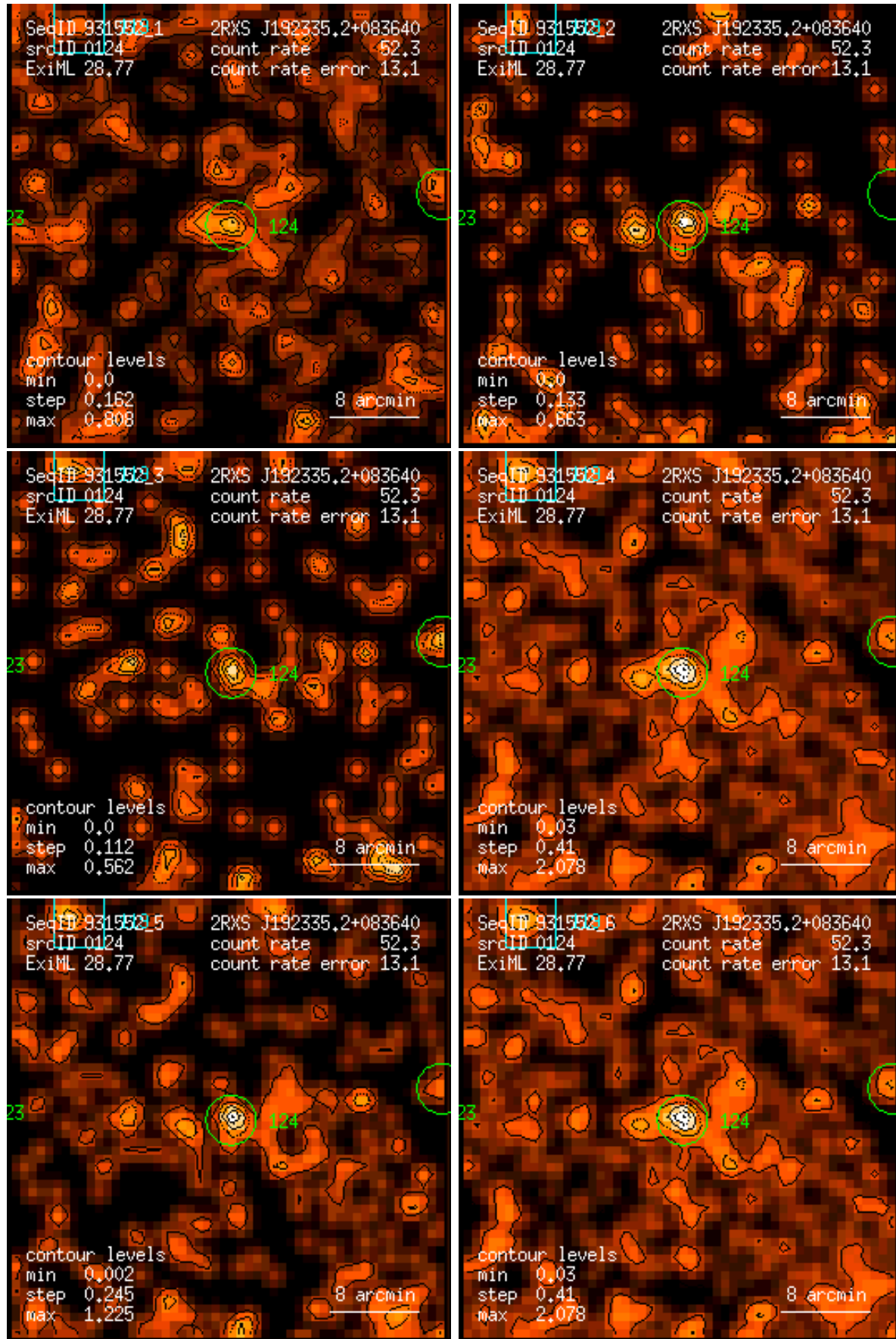
Figure 124: RASS 931552: detection 0124: band rate images, Gaussian filter: (1) PSPC channels 11 – 41, (2) 52 – 90, (3) 91 – 201, (4) 11 – 235, (5) 52 – 201, (6) 11 – 201. Broad band rates in counts/ks. Band rate contour levels in counts/ks/arcmin 2 .
