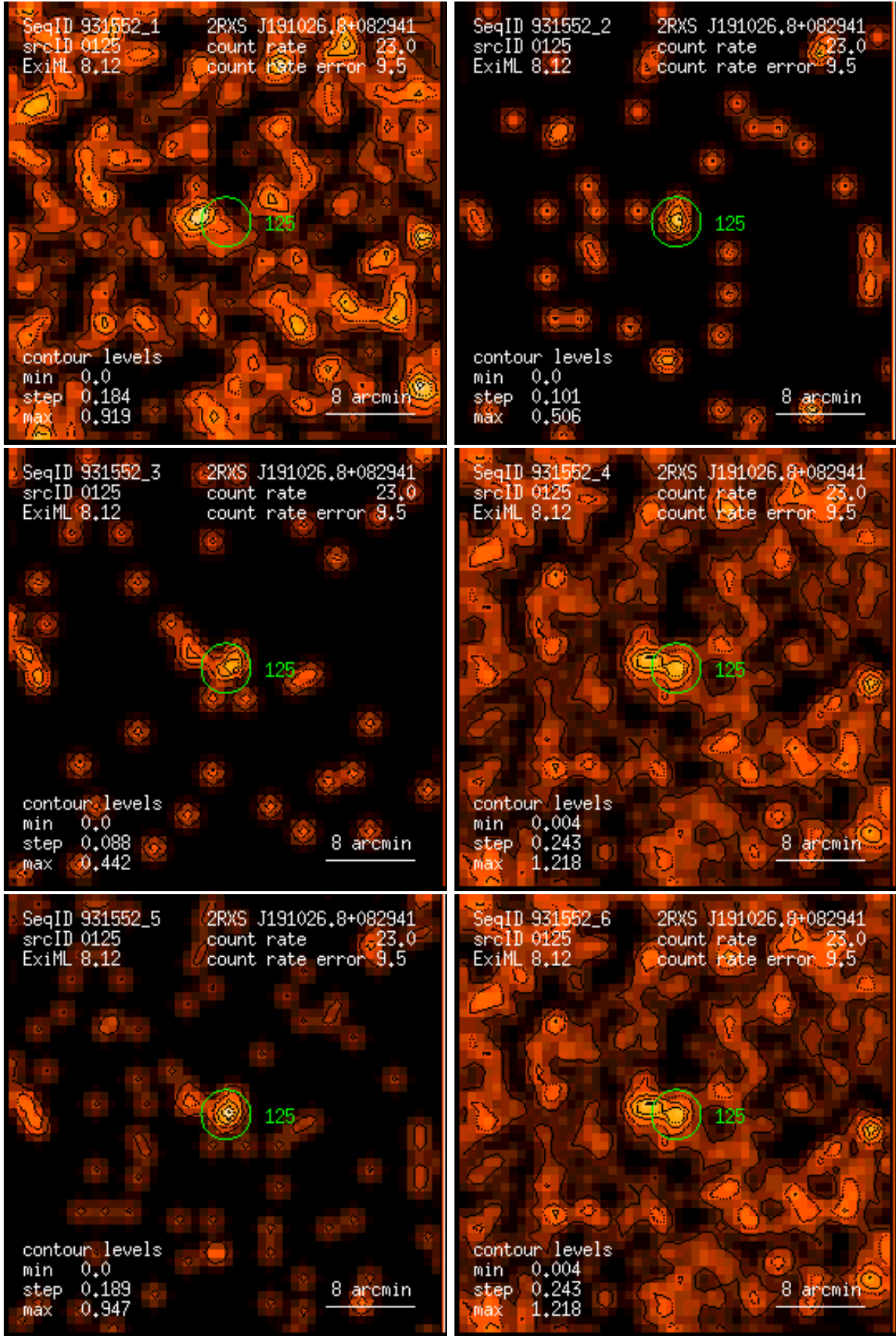
Figure 125: RASS 931552: detection 0125: band rate images, Gaussian filter: (1) PSPC channels 11 – 41, (2) 52 – 90, (3) 91 – 201, (4) 11 – 235, (5) 52 – 201, (6) 11 – 201. Broad band rates in counts/ks. Band rate contour levels in counts/ks/arcmin 2 .
