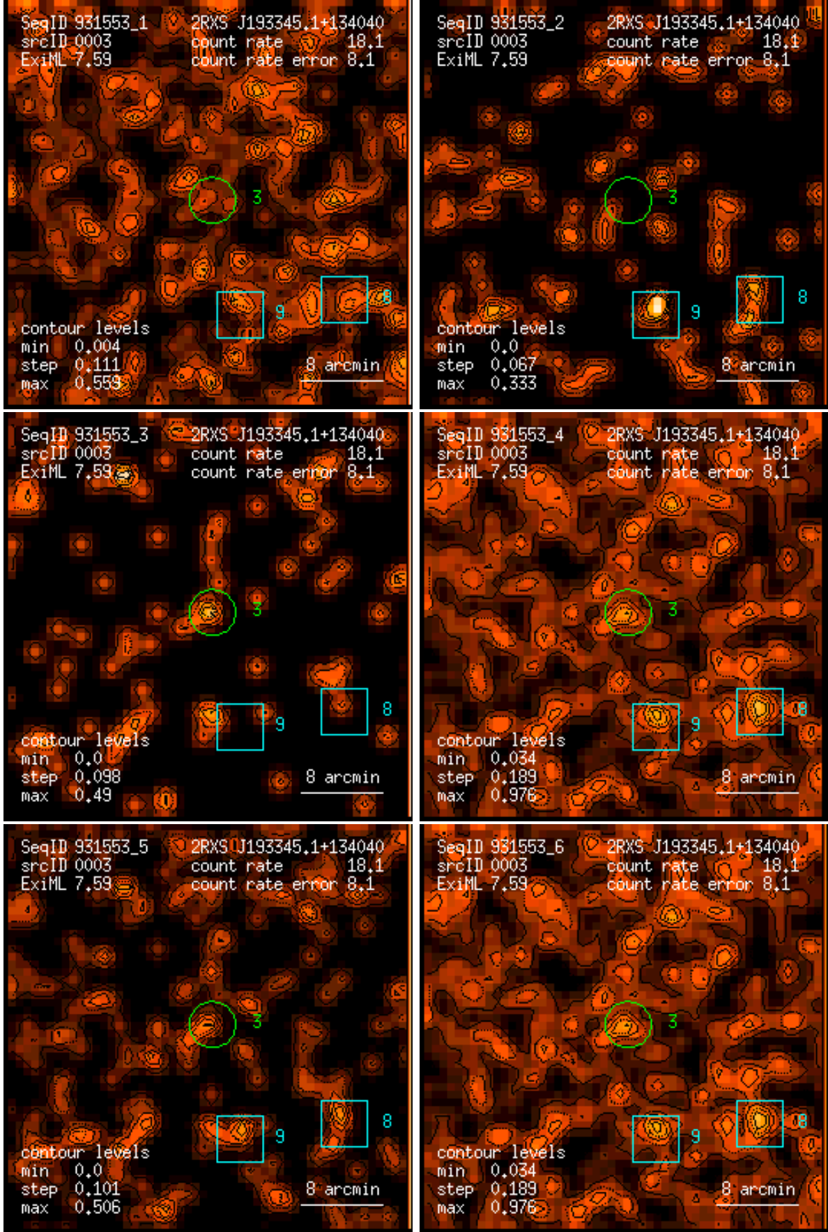
Figure 3: RASS 931553: detection 0003: band rate images, Gaussian filter: (1) PSPC channels 11 – 41, (2) 52 – 90, (3) 91 – 201, (4) 11 – 235, (5) 52 – 201, (6) 11 – 201. Broad band rates in counts/ks. Band rate contour levels in counts/ks/arcmin 2 .
